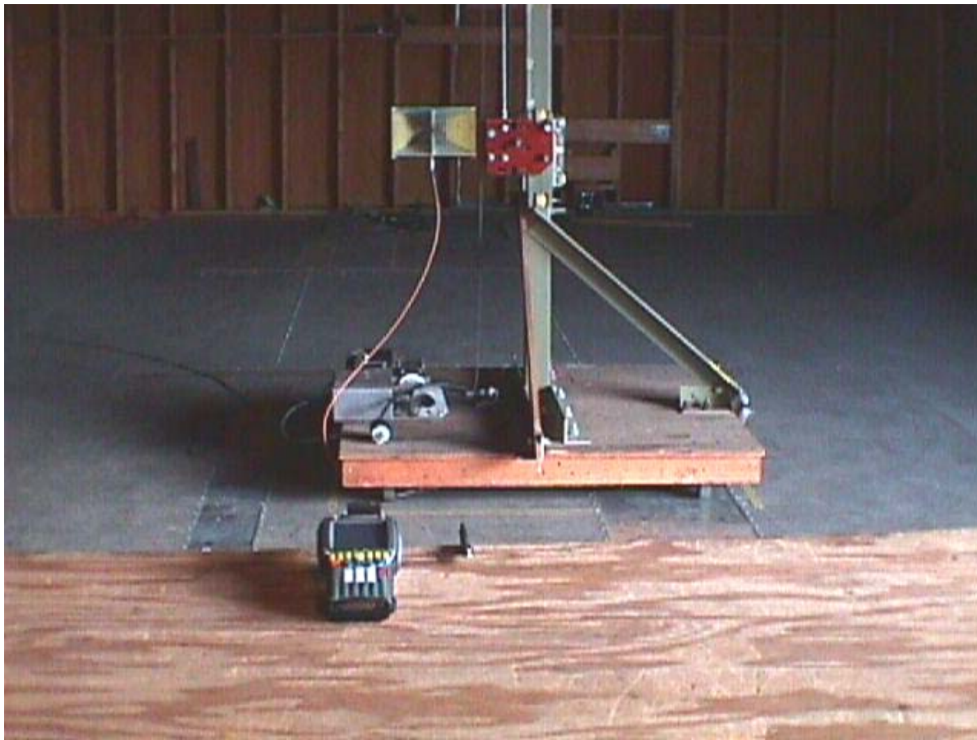
Test Configuration #1: Psion Teklogix Model RA2020 + Radiall/Larsen Antenna, Model EPA 02-016, Gain: 2 dBi
