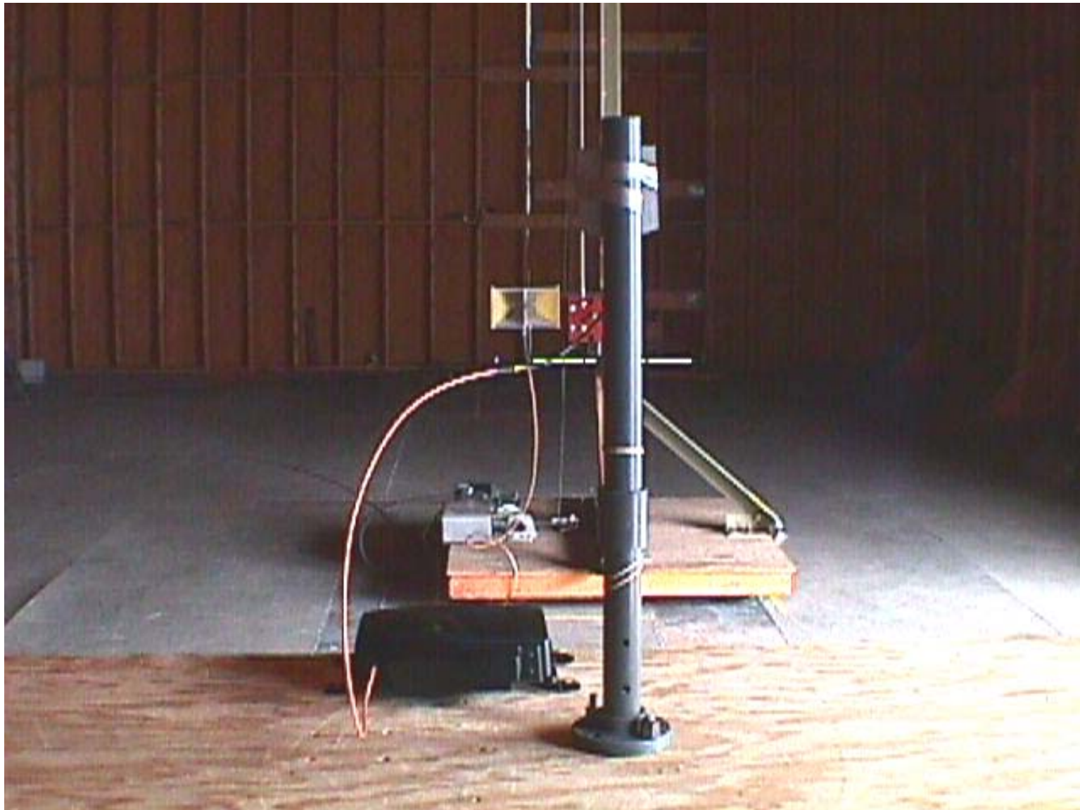
Test Configuration #5: Psion Teklogix Model No.: 9150-RA2020 + Cushcraft, Model S2307AMP10SMF, Gain: 7.5 dBi
