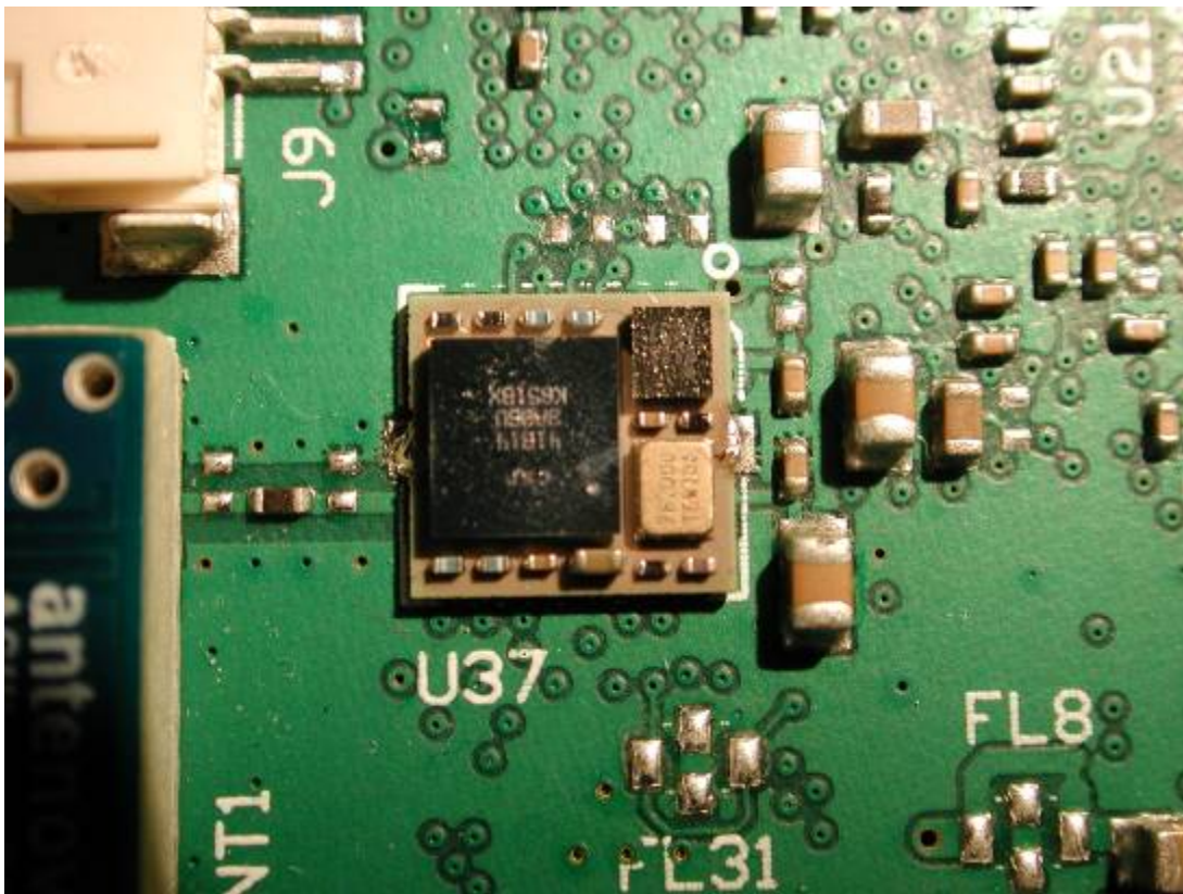
Bluetooth radio with shield removed U37
