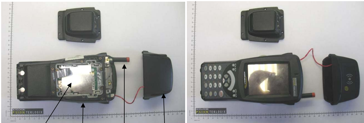
GPRS RA3030-G2 BlueTooth On the GPRS RFID Module Main Logic Board Antenna (Native in the WAP G2)
