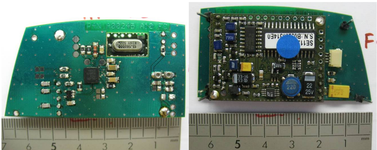
RFID MODULE HF-T2-G2: Mother Board with TAGSYS module
