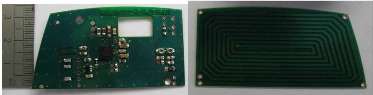
RFID MODULE HF-T2-G2: Mother Board with TAGSYS module
