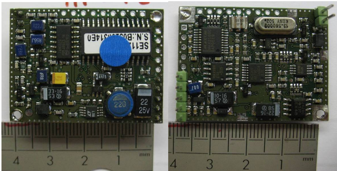
RFID MODULE HF-T2-G2: Mother Board without TAGSYS module
