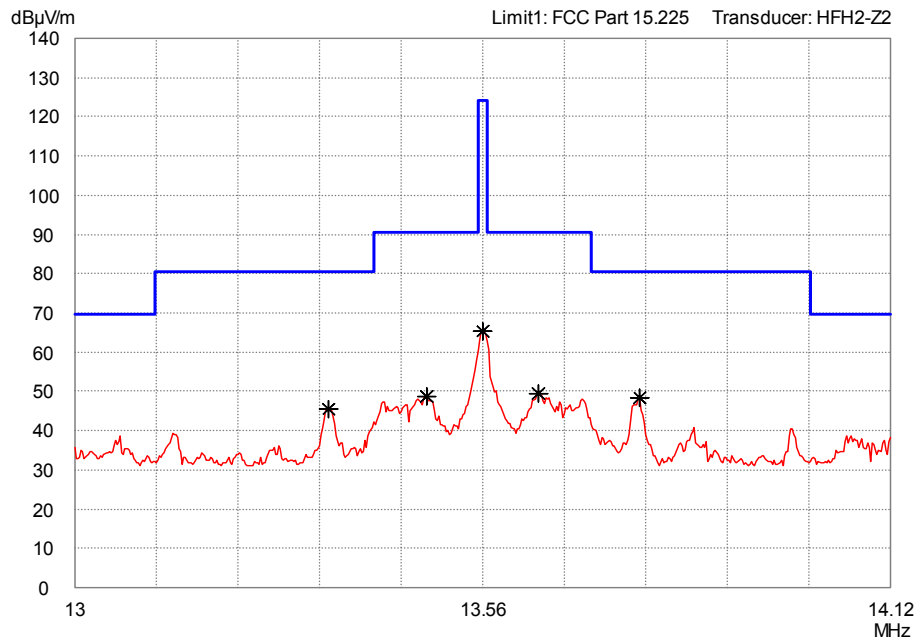
Figure 1: RBW = 10 kHz
