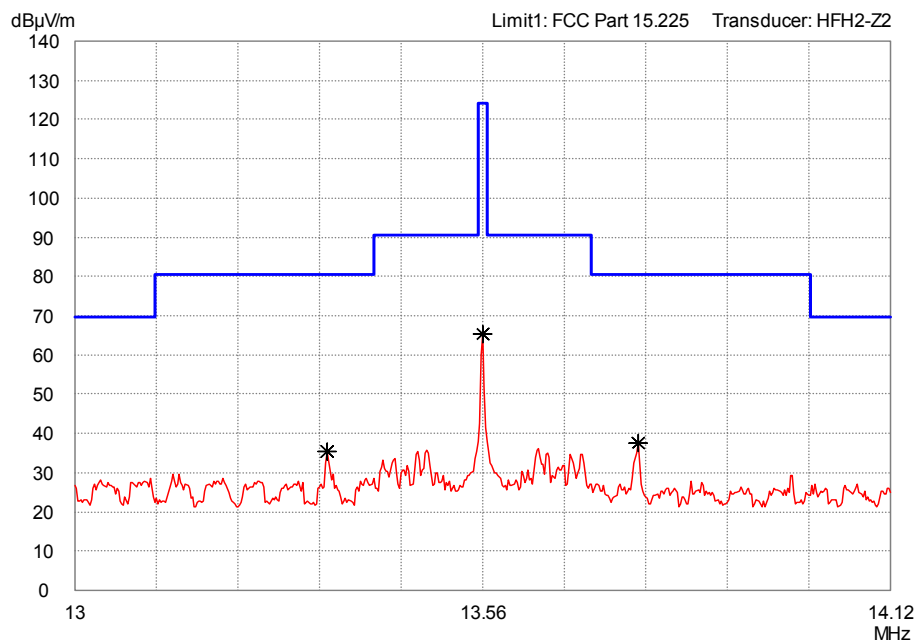
Figure 2: RBW = 1 kHz
