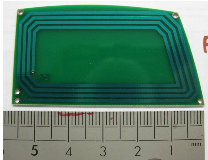
RFID MODULE HF-AM1-G2: Antenna
