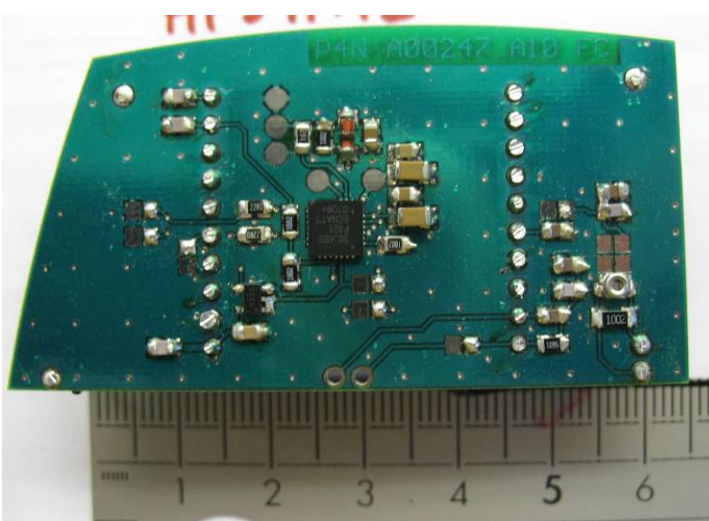
RFID MODULE HF-AM1-G2: Assembly
