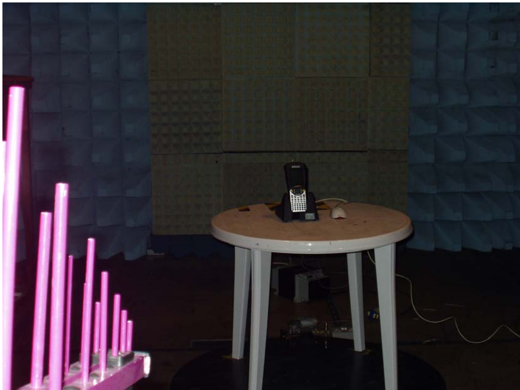
Photograph of the EUT (docked) as viewed from in front of the loop / horn antennas, site M.
