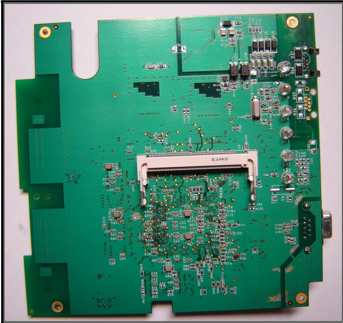
Photograph 21: Main PCB; Top View – Radio Removed
