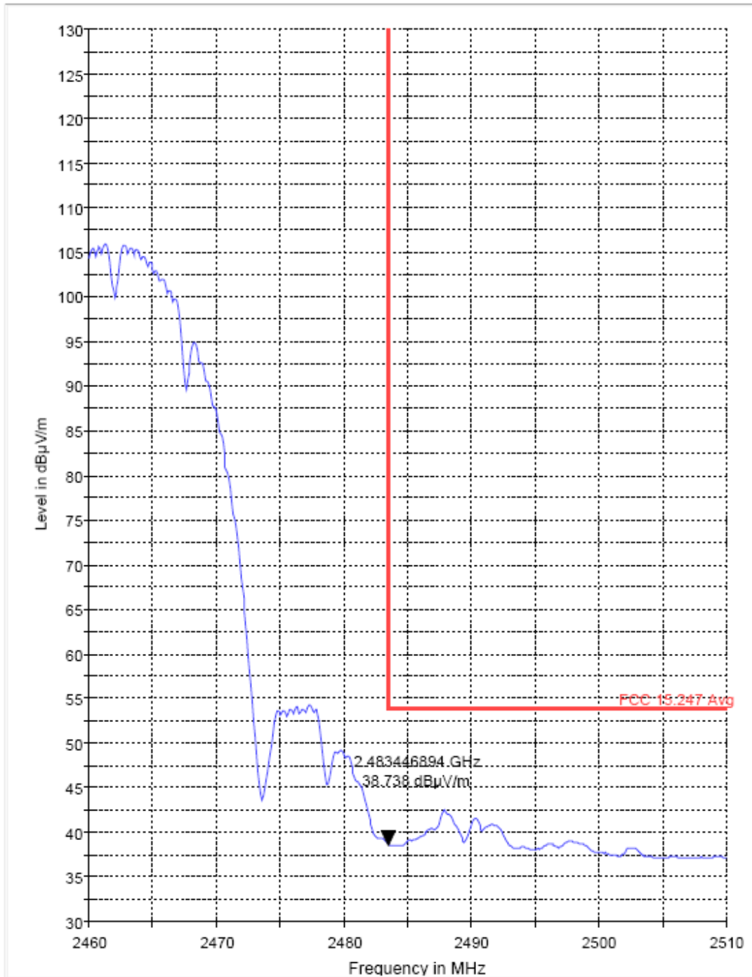
FCC 15.247 HBE Avg 3m
