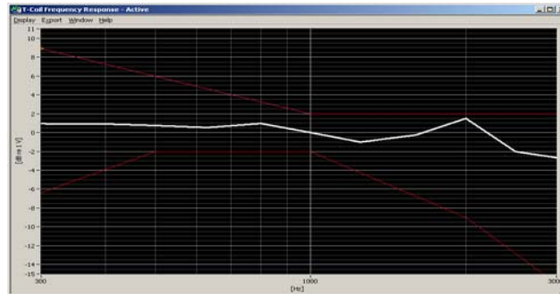
Figure 7-1 Axial Frequency Response
