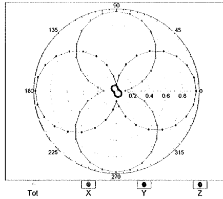
f=2200 MHz,R22,0°
