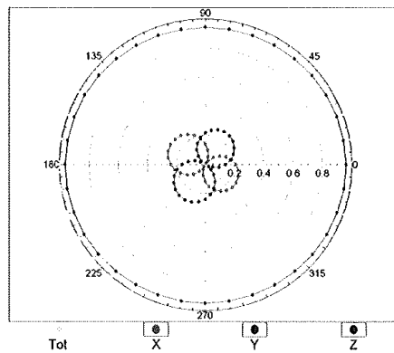
f=2200 MHz,R22,90°
