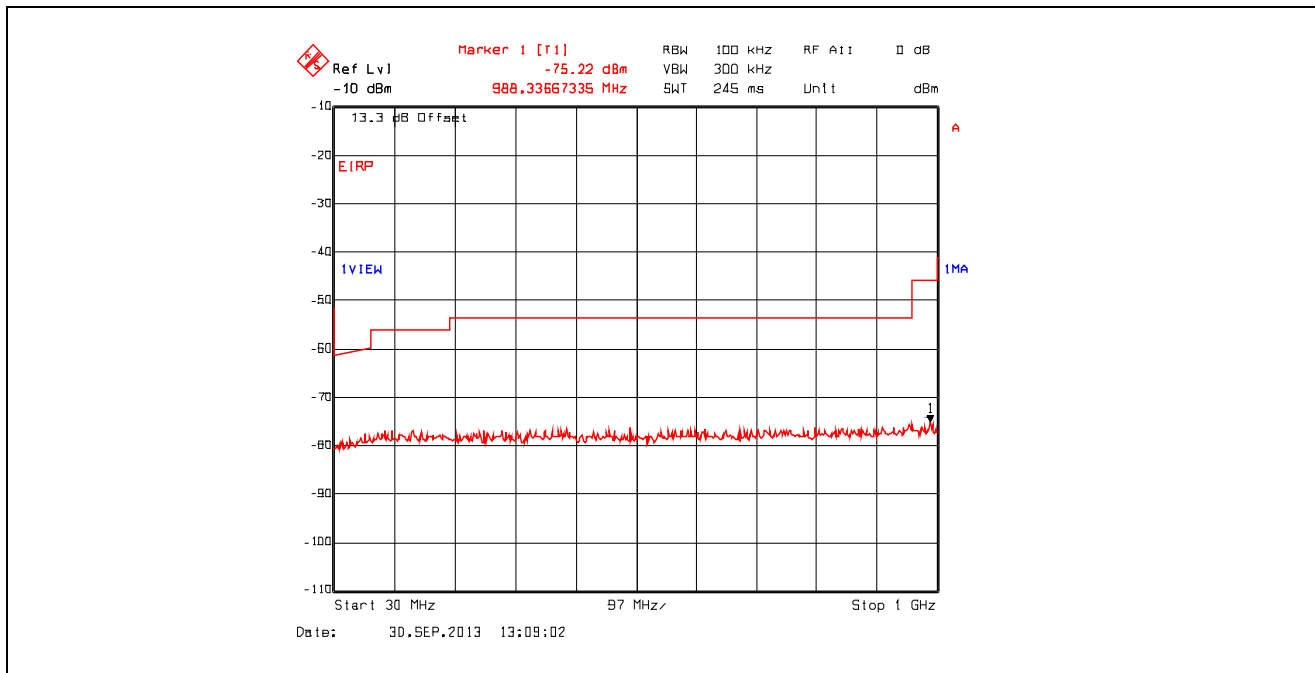
Plot 5.3.4.3.3. Conducted Spurious Emissions – Restricted Bands 802.11b, 1 Mbps Data Rate, 2472 MHz, 5 dBm Power Setting, 30 MHz - 1 GHz, Peak Detector
