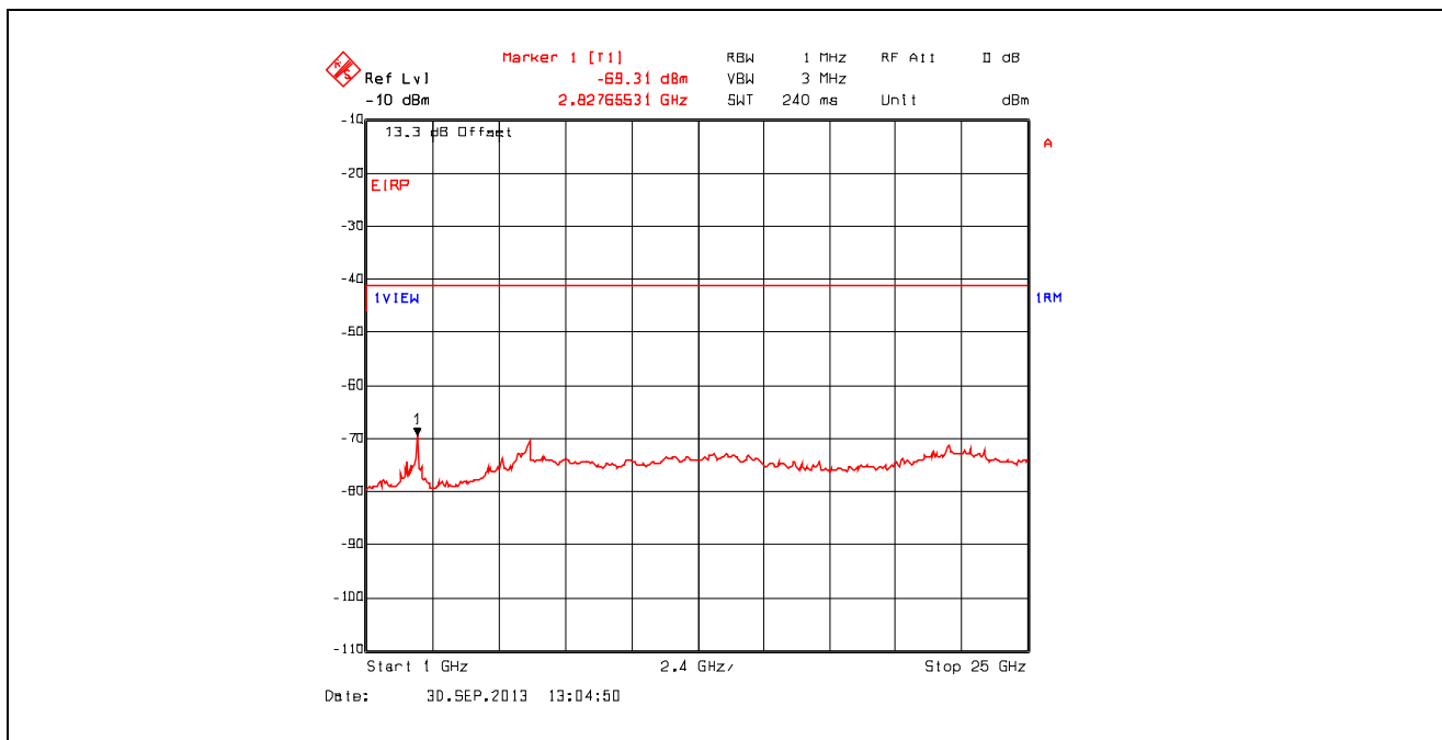
Plot 5.3.4.3.4. Conducted Spurious Emissions – Restricted Bands 802.11b, 1 Mbps Data Rate, 2472 MHz, 5 dBm Power Setting, 1 GHz - 25 GHz, Power Average (RMS) Detector
