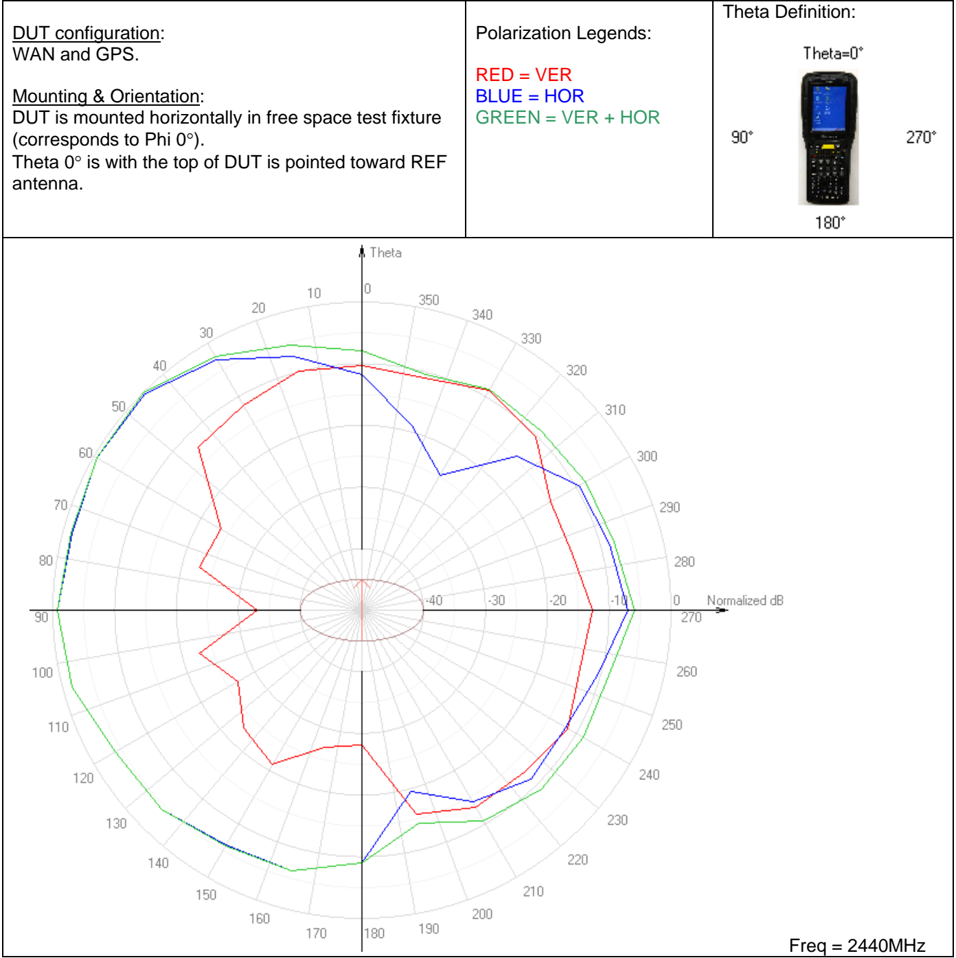
Figure 3: Measured Antenna Pattern @ Phi 0°
