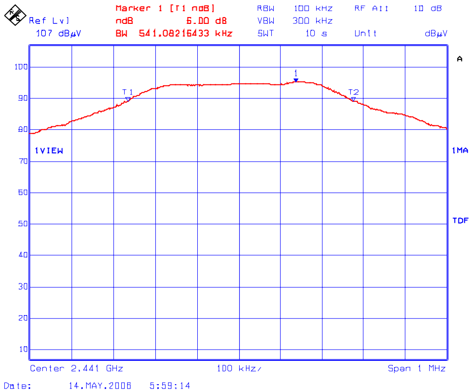
Plot 5.6.5.2.2: 6 dB Bandwidth Test Frequency: 2441 MHz
