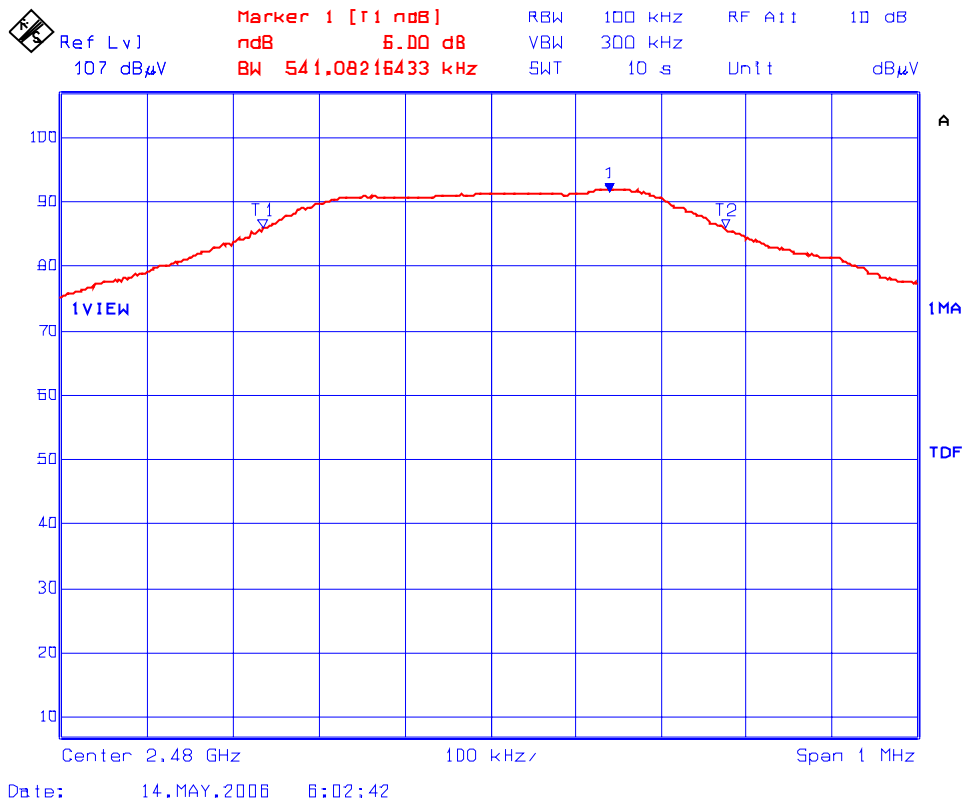
Plot 5.6.5.2.3: 6 dB Bandwidth Test Frequency: 2480 MHz
