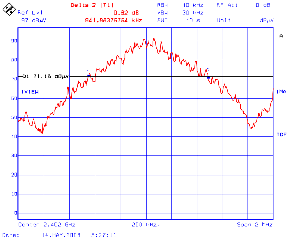
Plot 5.6.5.1.1: 20 dB Bandwidth Test Frequency: 2402 MHz
