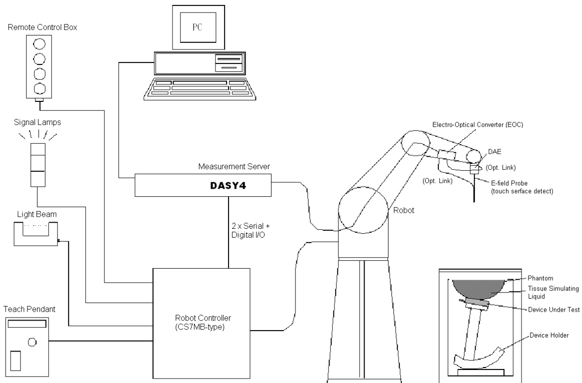
Fig. 5.1 DASY4 System
