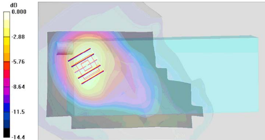
0 dB = 0.496mW/g
