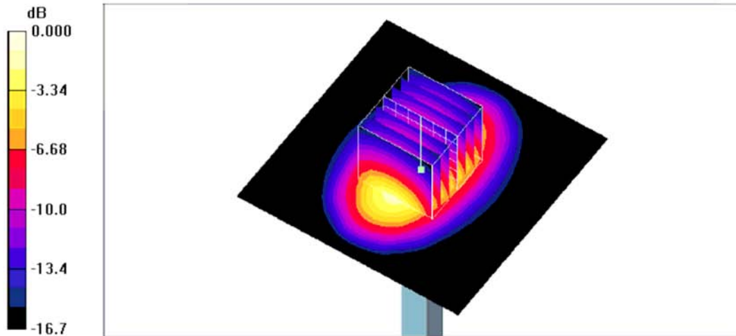
0 dB = 4.45mW/g
