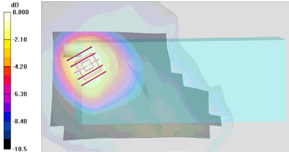
0 dB = 1.30mW/g
