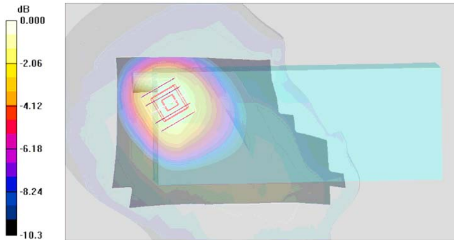
0 dB = 1.33mW/g
