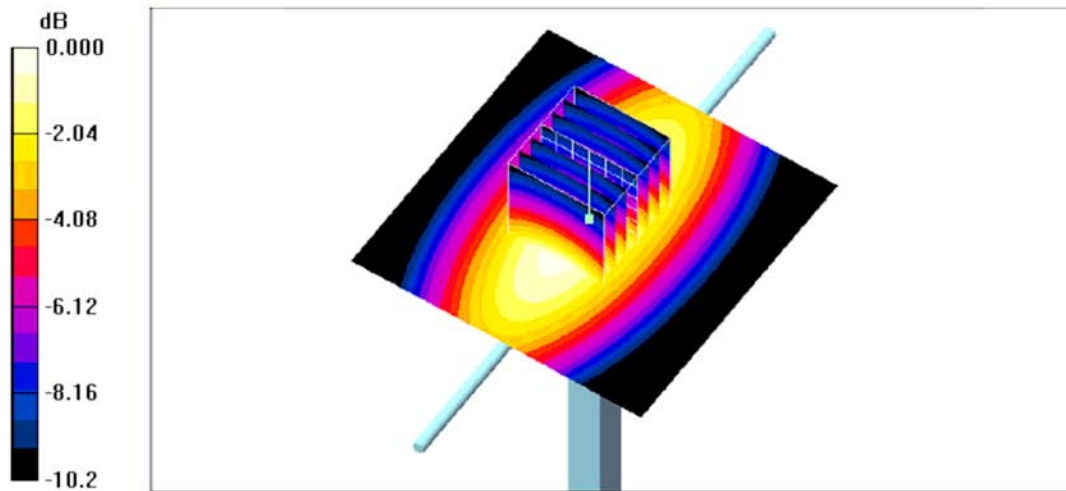
0 dB = 1.04mW/g
