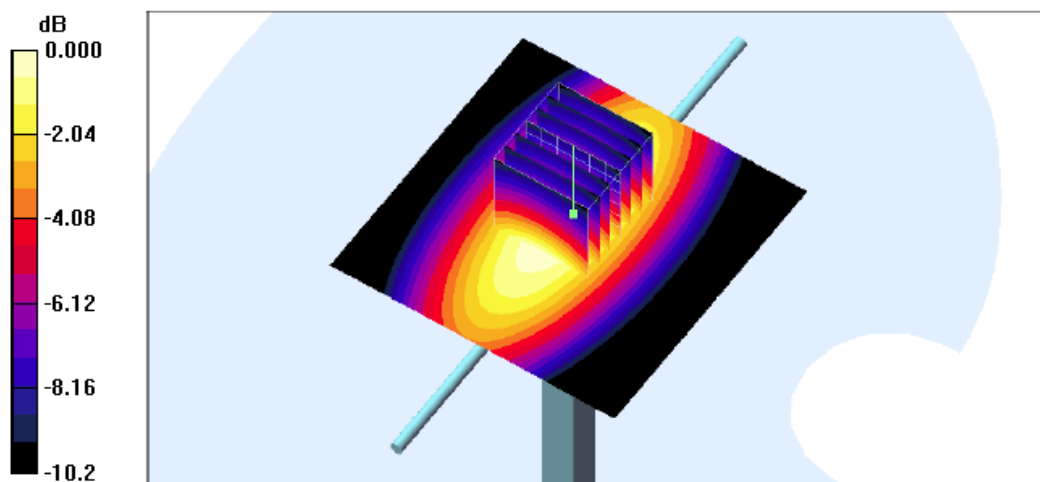
0 dB = 1.02mW/g
