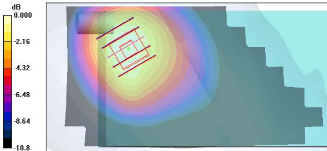
0 dB = 1.19mW/g
