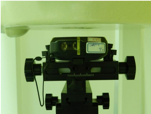
Front of the DUT with Phantom 1.5 cm Gap (DUT with Charger Snap Module 1)
