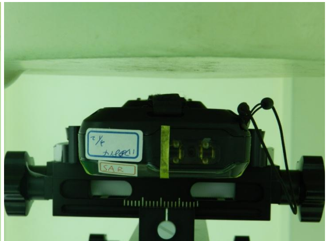
Back of the DUT with Phantom 1.5 cm Gap (DUT with Charger Snap Module 2)
