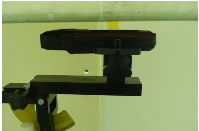
Front Face of the DUT with Phantom 1.5 cm Gap (DUT with Charger Snap Module 1)
