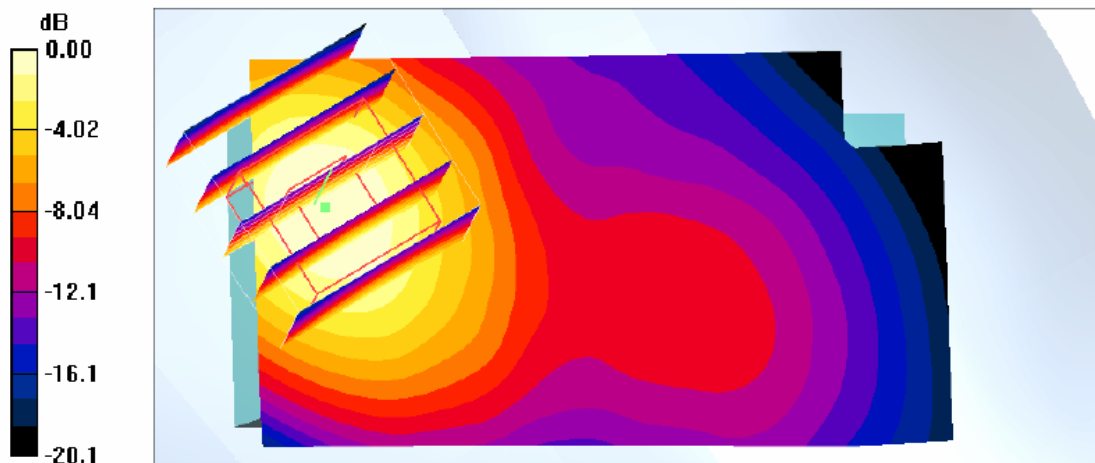
0 dB = 0.323mW/g
