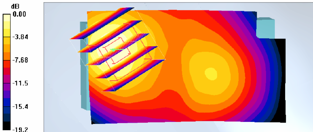
0 dB = 0.493mW/g
