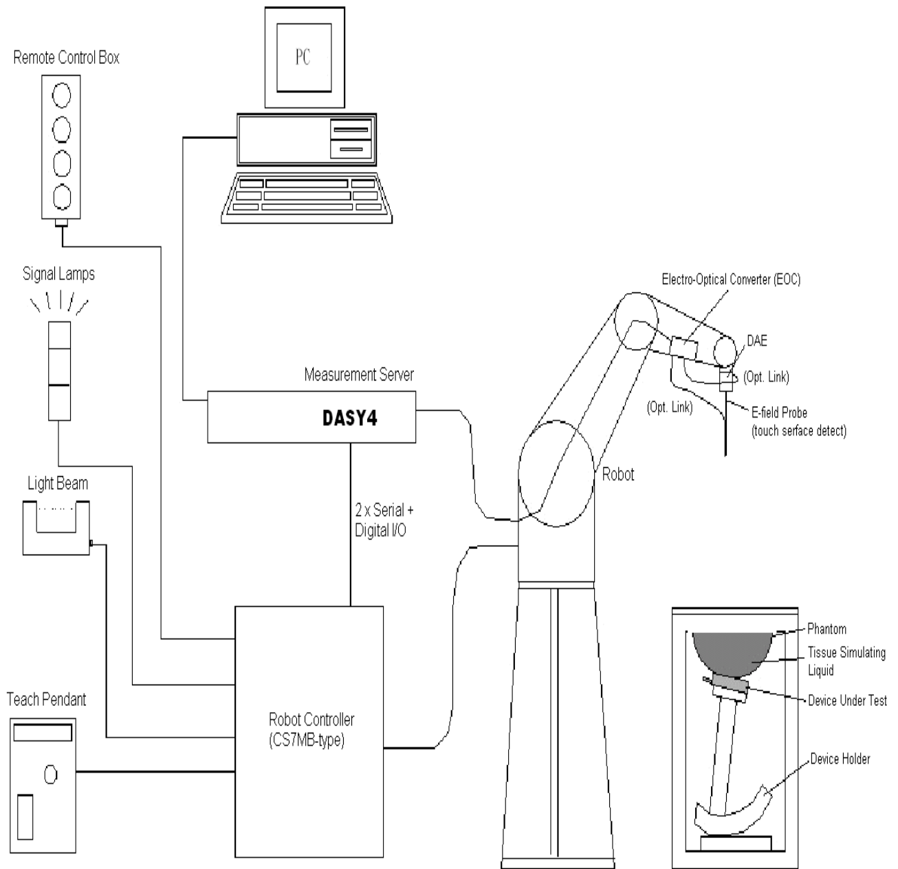
Fig. 5.1 DASY4 system
