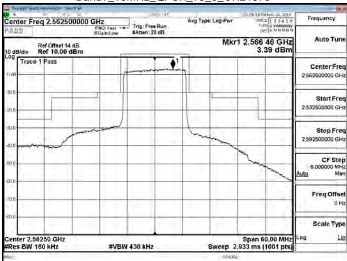
Band7_15MHz_QPSK_75_0_CH21375
