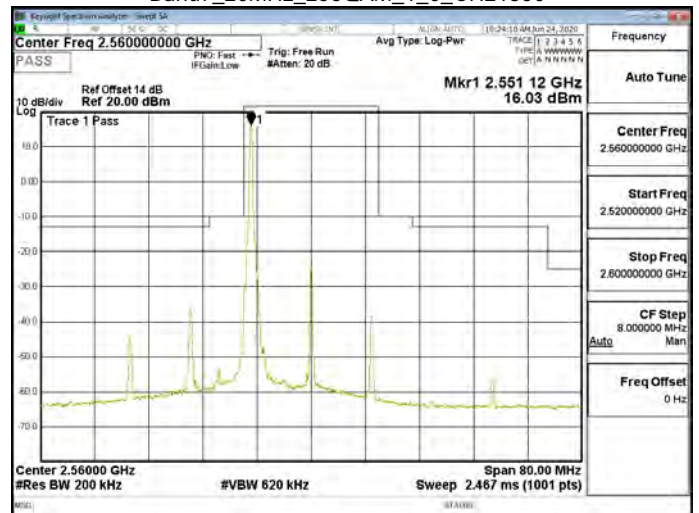
Band7_20MHz_256QAM_1_0_CH21350
