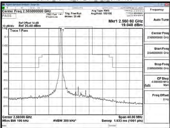
Band7_10MHz_64QAM_1_0_CH21400
