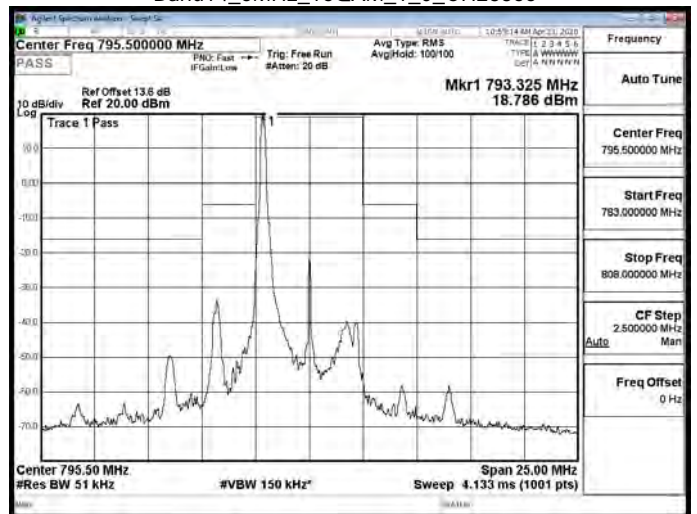
Band14_5MHz_16QAM_1_0_CH23355
