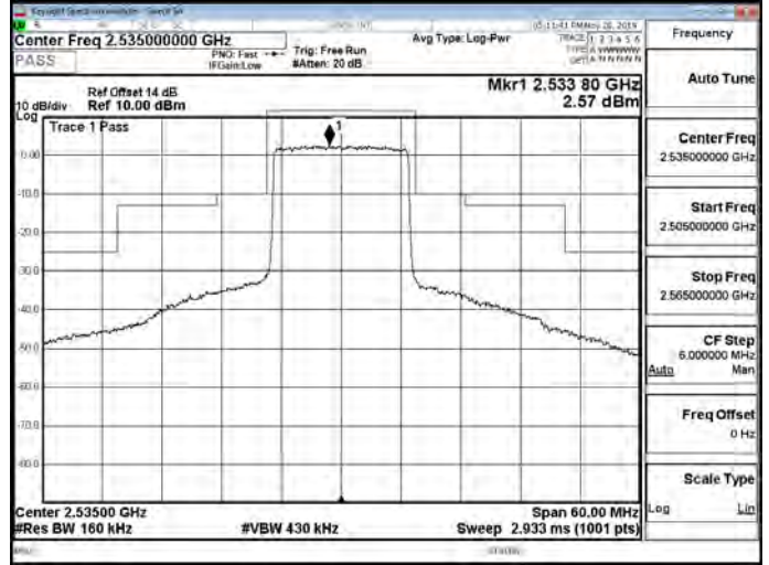
Band7_15MHz_16QAM_75_0_CH21375
