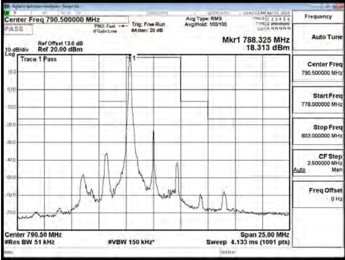
Band14_5MHz_64QAM_1_0_CH23330
