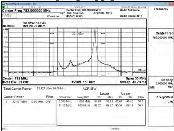
Band13_10MHz_QPSK_50_0_CH23230
