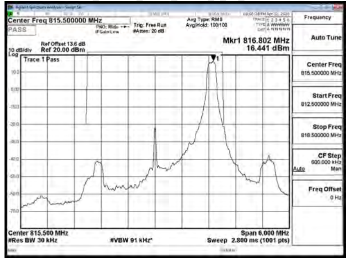
Band26_Part90s_3MHz_QPSK_1_14_CH26740
