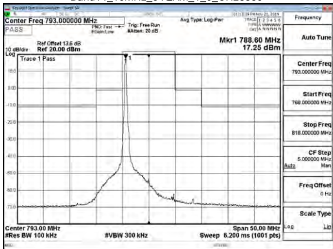
Band14_10MHz_64QAM_1_49_CH23330
