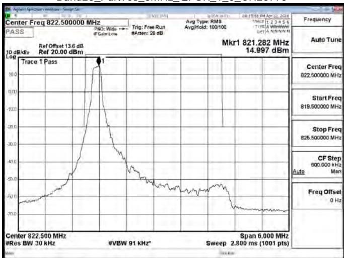
Band26_Part90s_3MHz_QPSK_1_0_CH26775
