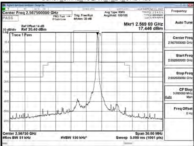
Band7_5MHz_16QAM_1_24_CH21425
