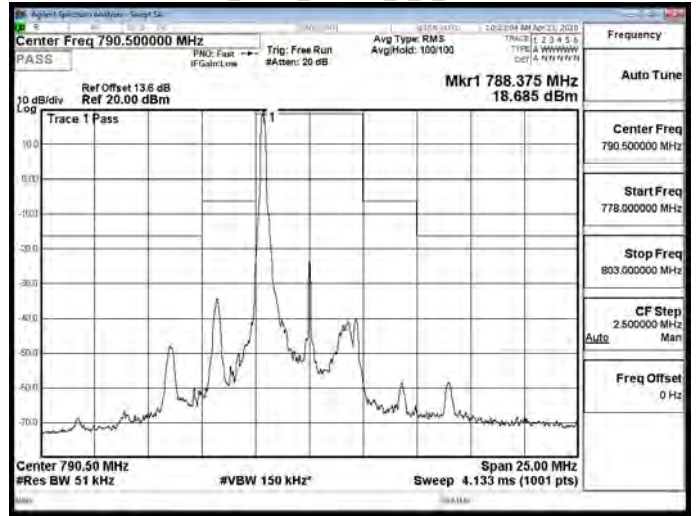
Band14_5MHz_16QAM_1_0_CH23330
