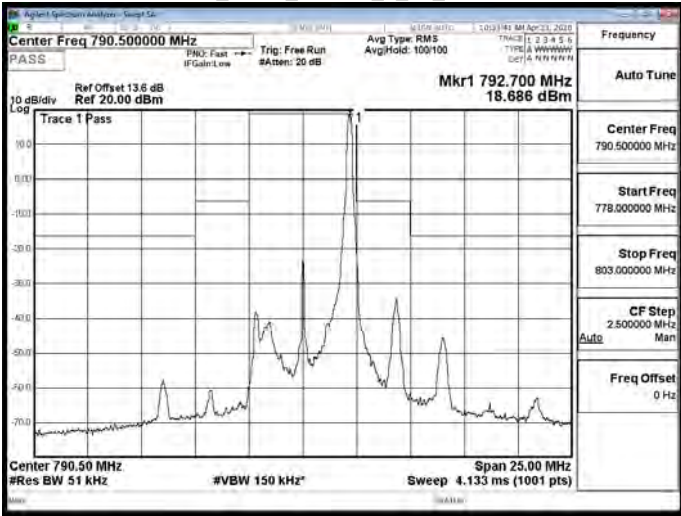
Band14_5MHz_16QAM_1_24_CH23330
