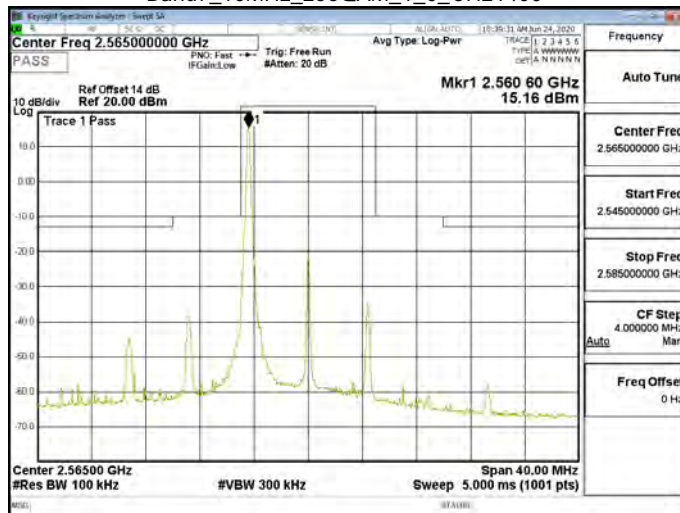
Band7_10MHz_256QAM_1_0_CH21400
