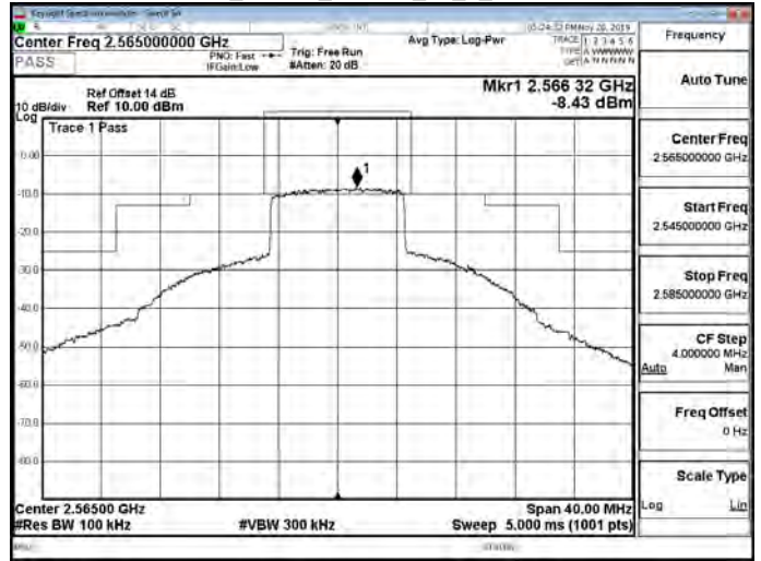
Band7_10MHz_16QAM_50_0_CH21400
