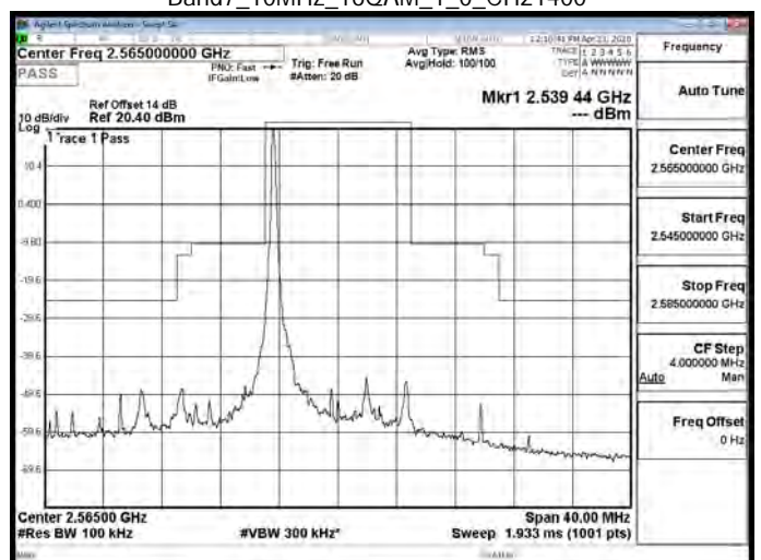
Band7_10MHz_16QAM_1_0_CH21400
