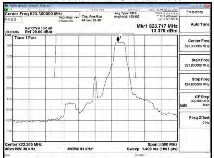
Band26_Part90s_1.4MHz_64QAM_1_5_CH26783
