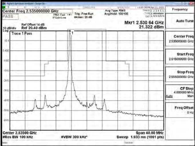
Band7_10MHz_QPSK_1_0_CH21400
