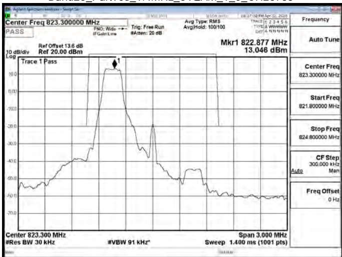
Band26_Part90s_1.4MHz_64QAM_1_0_CH26783
