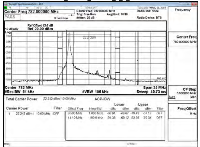
Band13_10MHz_16QAM_1_49_CH23230
