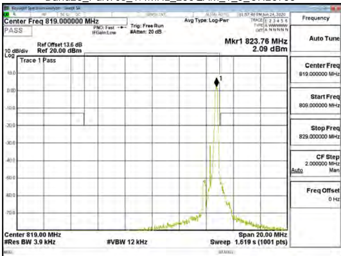
Band26_Part90s_1.4MHz_256QAM_1_5_CH26783
