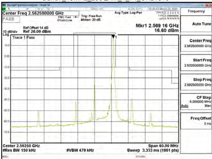
Band7_15MHz_256QAM_1_74_CH21375
