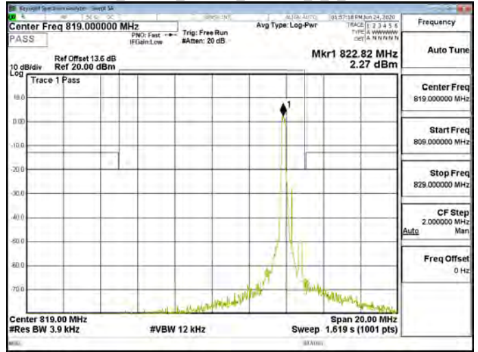
Band26_Part90s_1.4MHz_256QAM_1_0_CH26783
