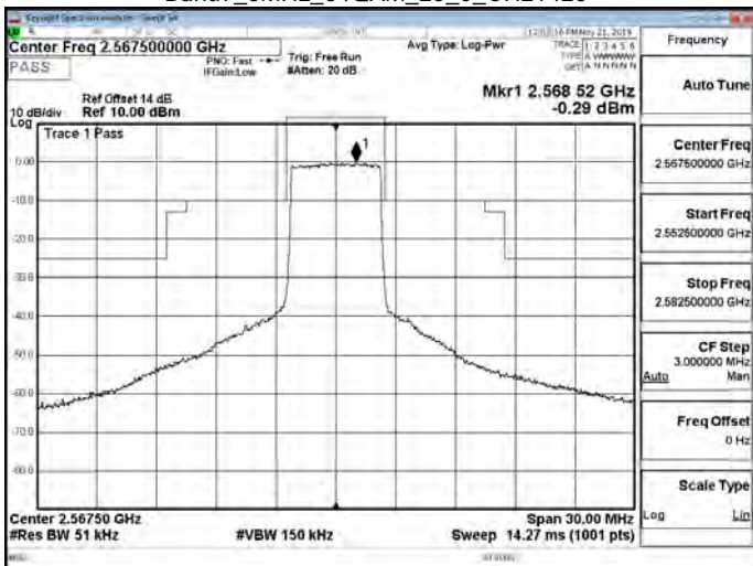
Band7_5MHz_64QAM_25_0_CH21425
