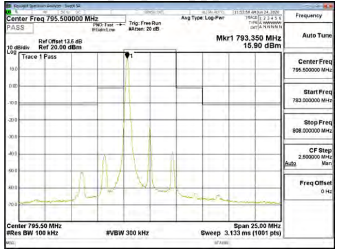
Band14_5MHz_256QAM_1_0_CH23355
