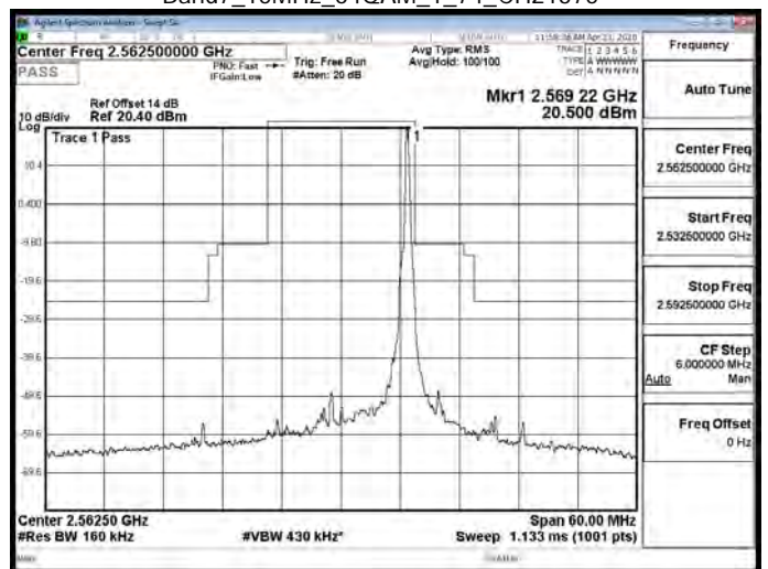
Band7_15MHz_64QAM_1_74_CH21375
