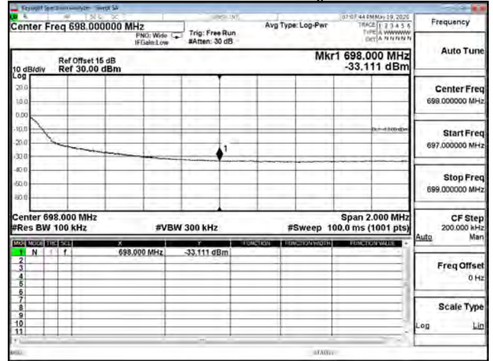
LTE\Band71_20MHz_QPSK_100_0_High CH133372-688
