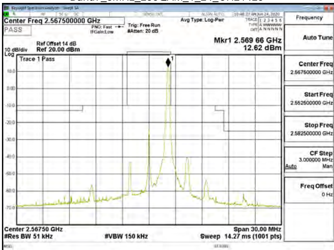
Band7_5MHz_256QAM_1_24_CH21425
