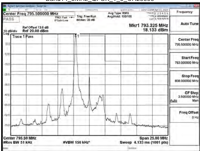
Band14_5MHz_QPSK_1_0_CH23355
