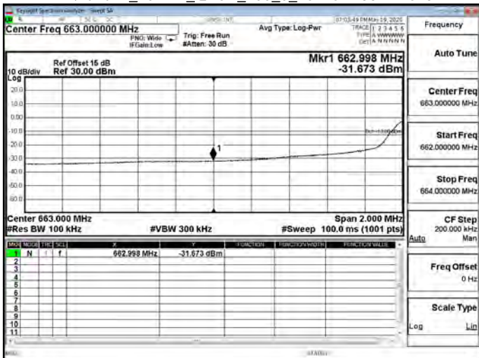
LTE\Band71_20MHz_QPSK_100_0_Low CH133222-673
