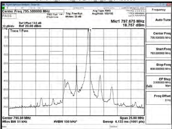
Band14_5MHz_16QAM_1_24_CH23355
