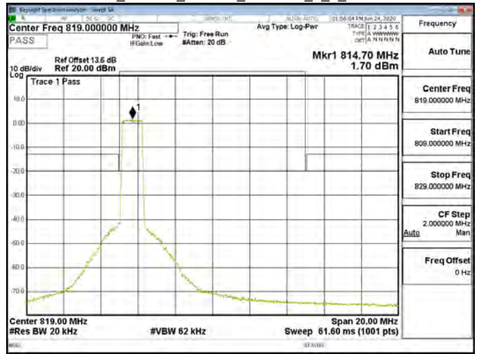
Band26_Part90s_1.4MHz_256QAM_6_0_CH26740
