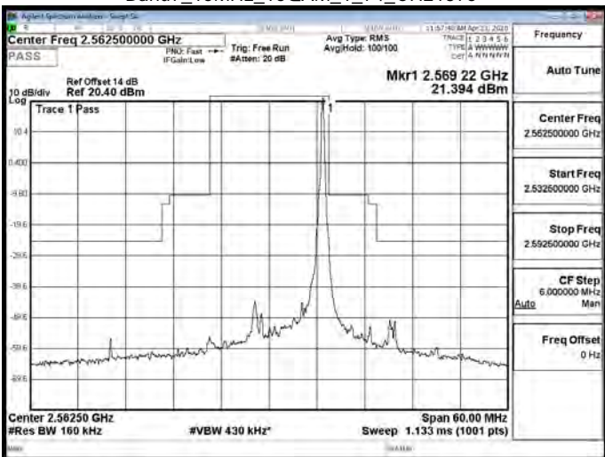
Band7_15MHz_16QAM_1_74_CH21375
