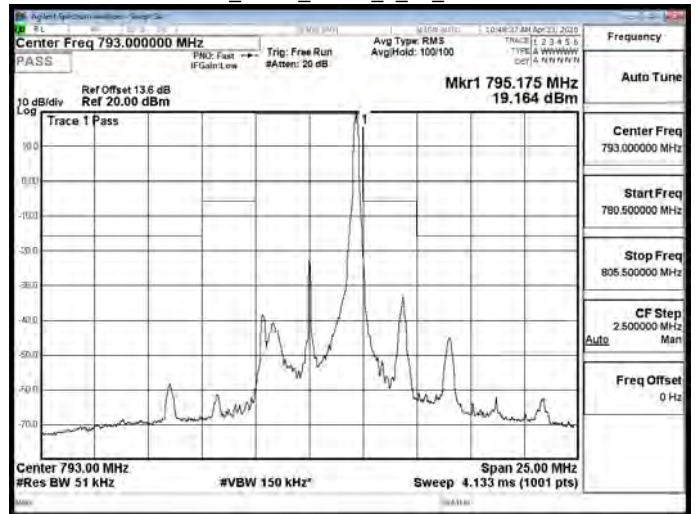
Band14_5MHz_QPSK_1_24_CH23355
