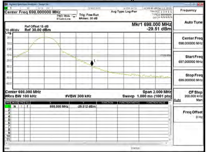
LTE\Band71_10MHz_QPSK_1_49_High CH133422-693
