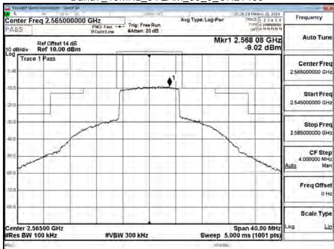
Band7_10MHz_64QAM_50_0_CH21400
