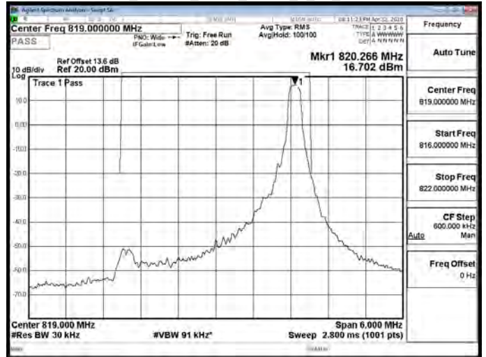
Band26_Part90s_3MHz_QPSK_1_14_CH26775
