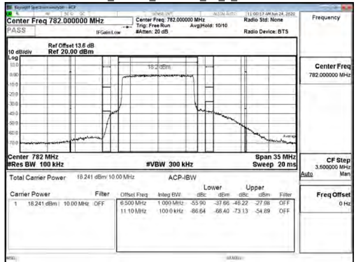
Band13_10MHz_256QAM_50_0_CH23230
