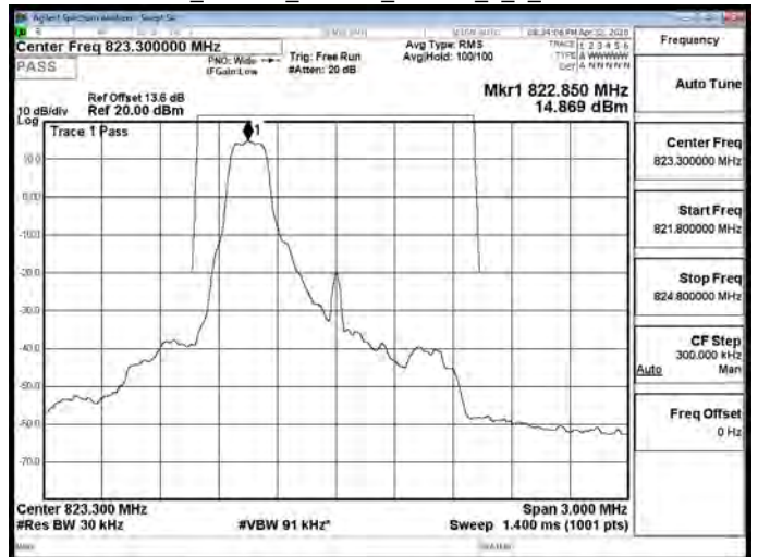
Band26_Part90s_1.4MHz_16QAM_1_0_CH26783
