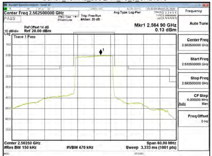
Band7_15MHz_256QAM_75_0_CH21375
