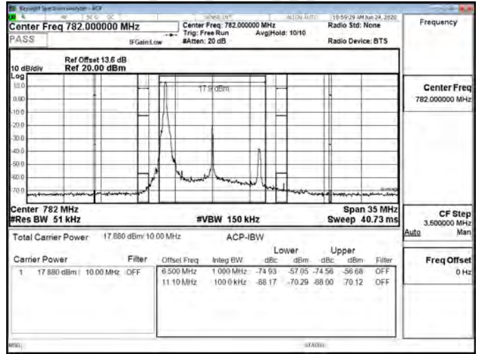
Band13_10MHz_256QAM_1_49_CH23230
