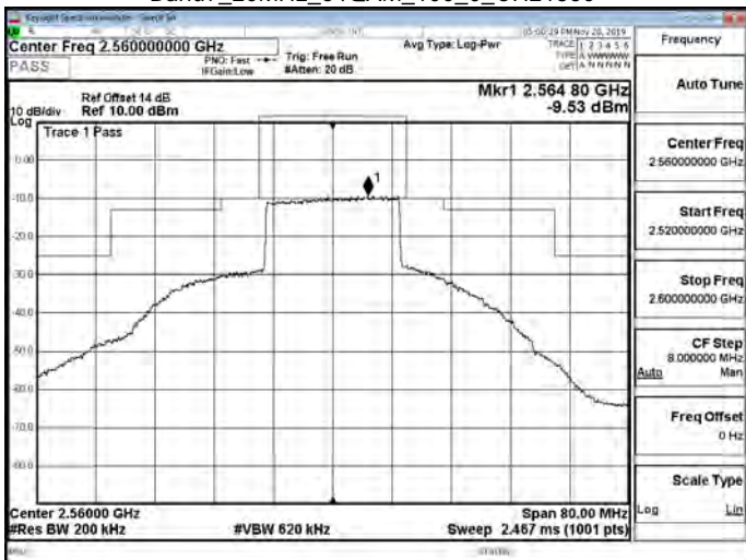
Band7_20MHz_64QAM_100_0_CH21350
