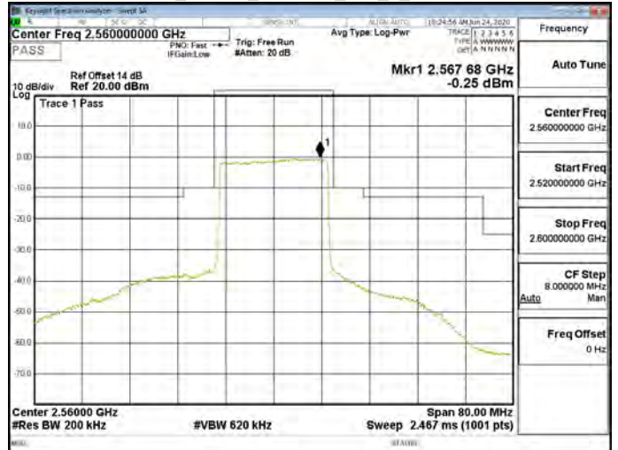
Band7_20MHz_256QAM_100_0_CH21350
