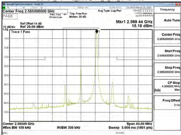
Band7_10MHz_256QAM_1_49_CH21400
