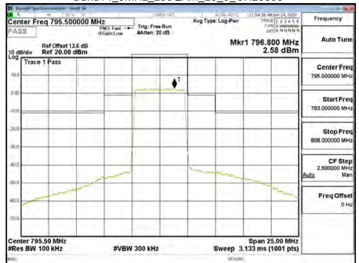
Band14_5MHz_256QAM_25_0_CH23355
