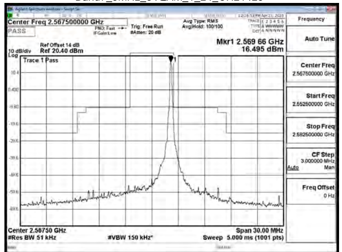
Band7_5MHz_64QAM_1_24_CH21425
