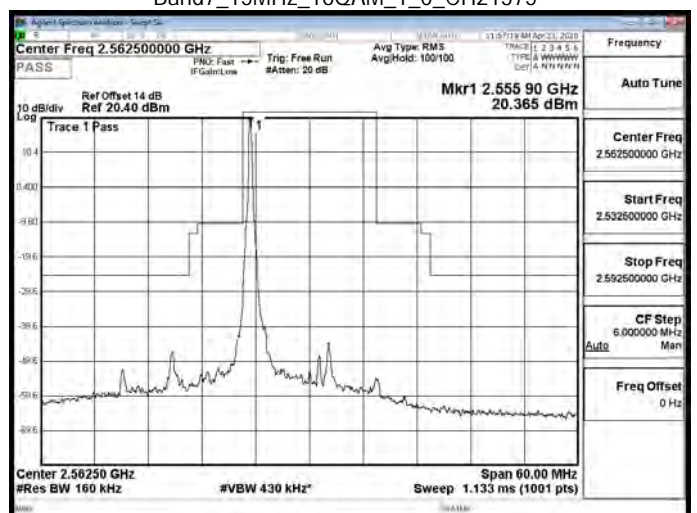
Band7_15MHz_16QAM_1_0_CH21375
