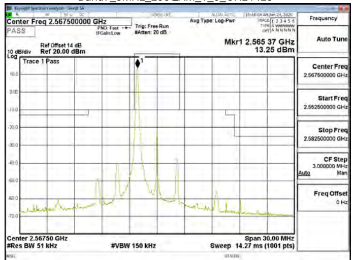
Band7_5MHz_256QAM_1_0_CH21425
