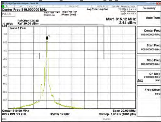
Band26_Part90s_1.4MHz_256QAM_1_5_CH26740
