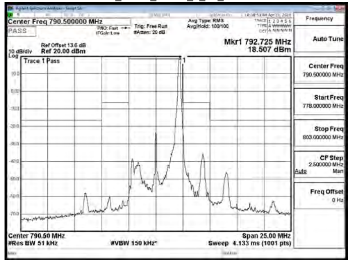
Band14_5MHz_QPSK_1_24_CH23330
