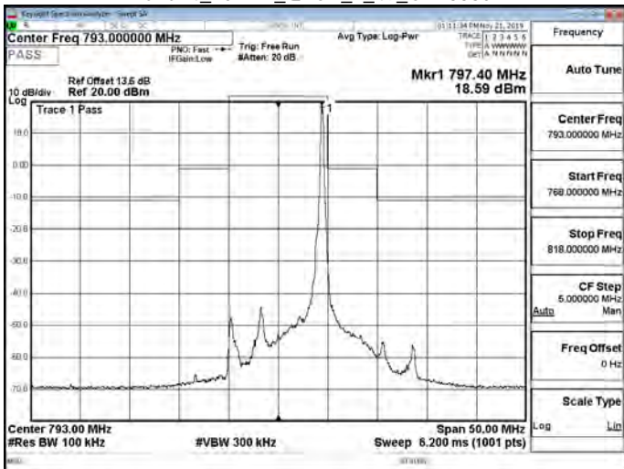
Band14_10MHz_QPSK_50_0_CH23330
