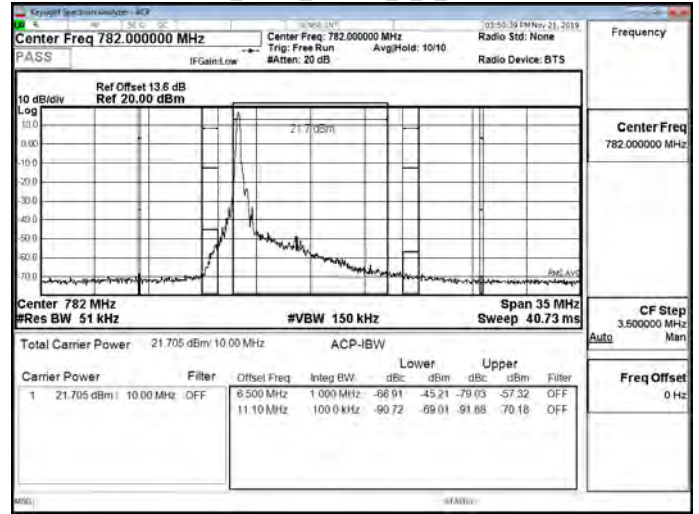
Band13_5MHz_16QAM_1_0_CH23230
