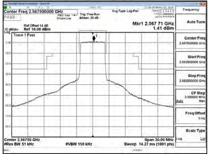
Band7_5MHz_16QAM_25_0_CH21425
