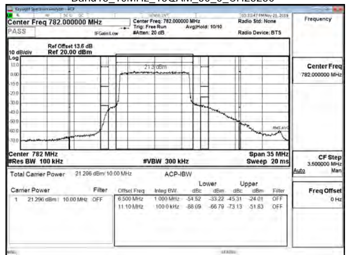
Band13_10MHz_16QAM_50_0_CH23230
