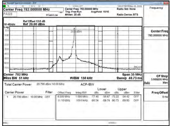
Band13_5MHz_QPSK_1_24_CH23230
