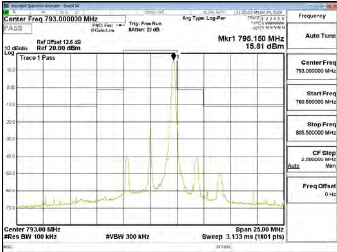
Band14_5MHz_256QAM_1_24_CH23355
