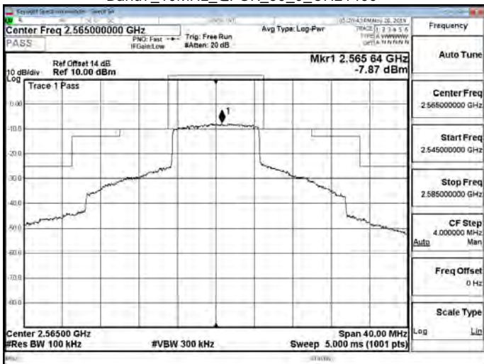
Band7_10MHz_QPSK_50_0_CH21400
