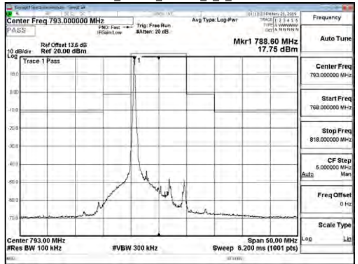
Band14_10MHz_16QAM_1_49_CH23330
