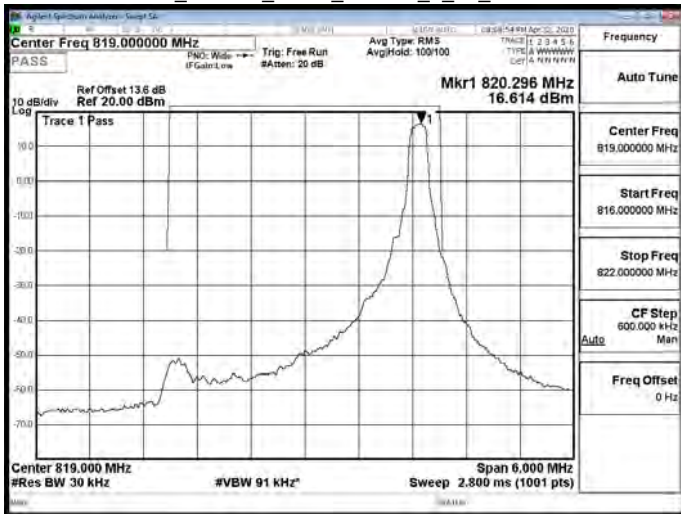
Band26_Part90s_3MHz_16QAM_1_14_CH26775
