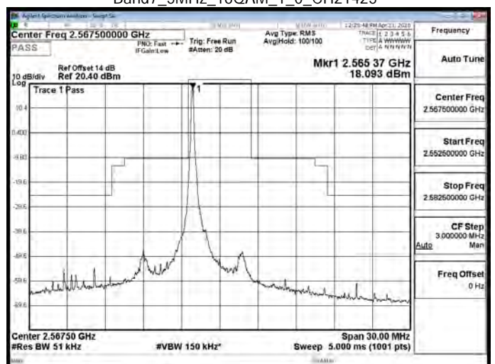
Band7_5MHz_16QAM_1_0_CH21425
