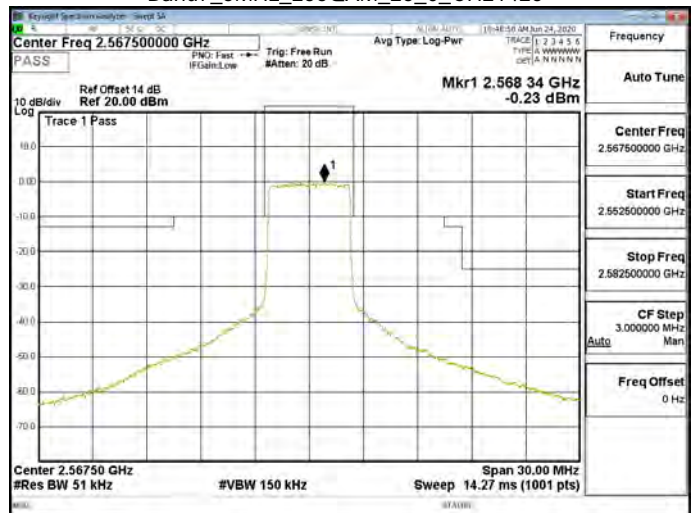
Band7_5MHz_256QAM_25_0_CH21425
