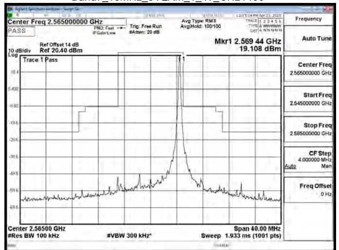
Band7_10MHz_64QAM_1_49_CH21400
