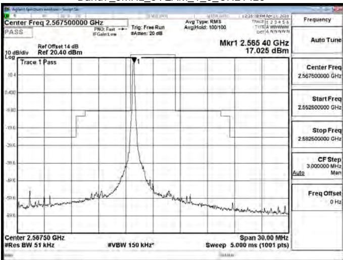
Band7_5MHz_64QAM_1_0_CH21425
