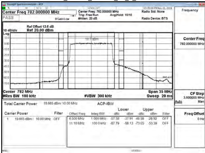
Band13_10MHz_64QAM_50_0_CH23230
