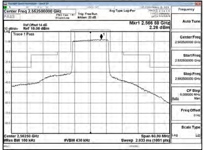
Band7_15MHz_16QAM_75_0_CH21375
