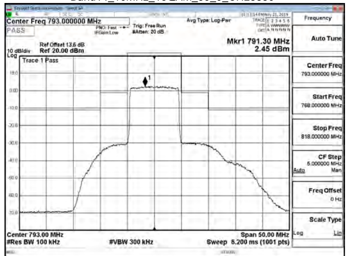
Band14_10MHz_16QAM_50_0_CH23330
