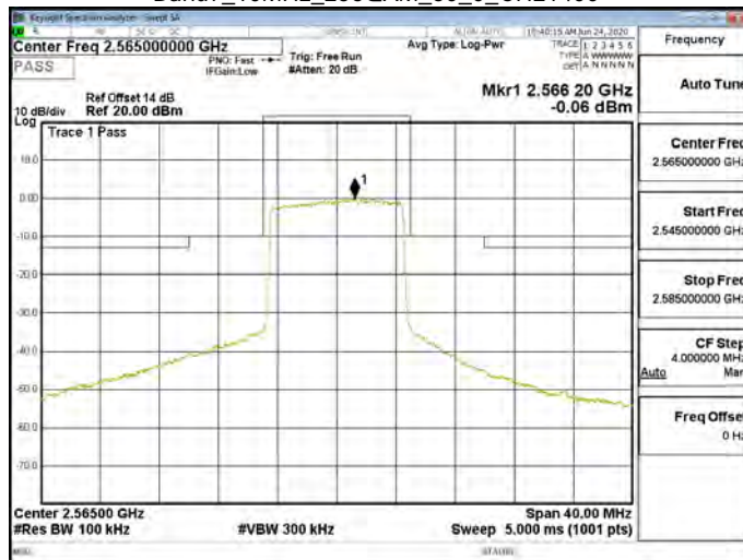
Band7_10MHz_256QAM_50_0_CH21400
