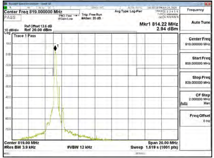
Band26_Part90s_1.4MHz_256QAM_1_0_CH26740
