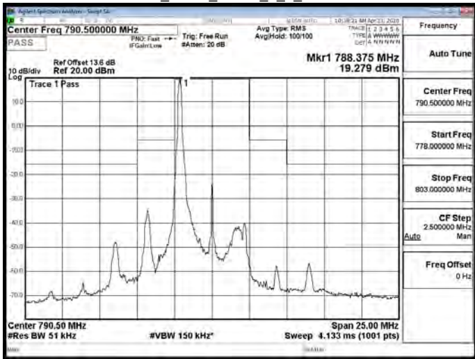
Band14_5MHz_QPSK_1_0_CH23330
