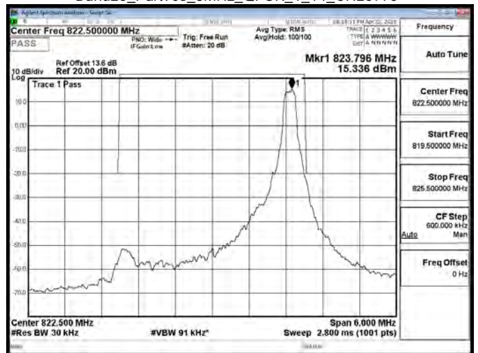
Band26_Part90s_3MHz_QPSK_1_14_CH26775
