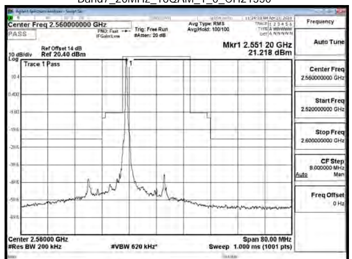
Band7_20MHz_16QAM_1_0_CH21350
