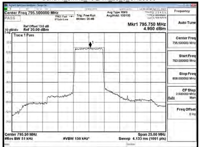
Band14_5MHz_16QAM_25_0_CH23355
