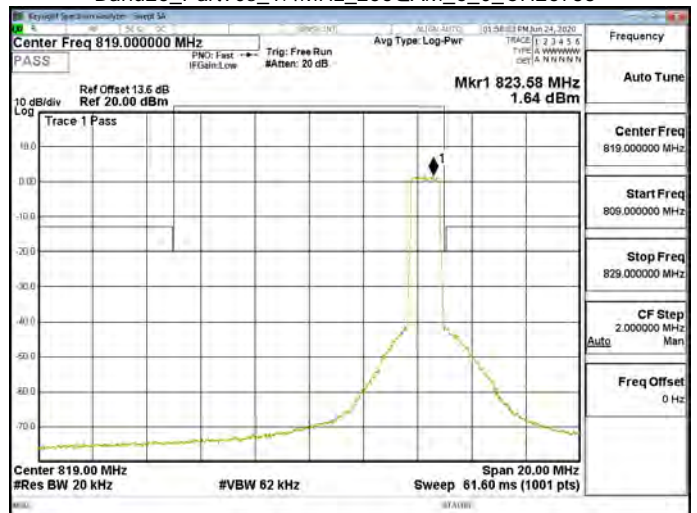
Band26_Part90s_1.4MHz_256QAM_6_0_CH26783
