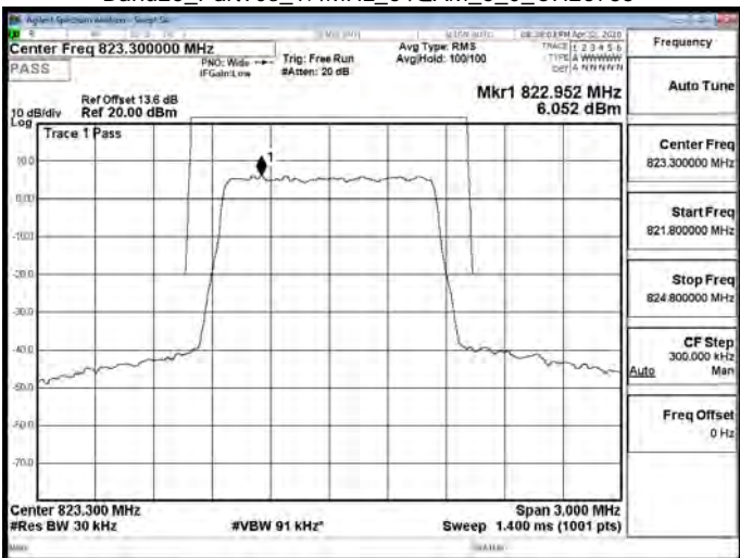
Band26_Part90s_1.4MHz_64QAM_6_0_CH26783
