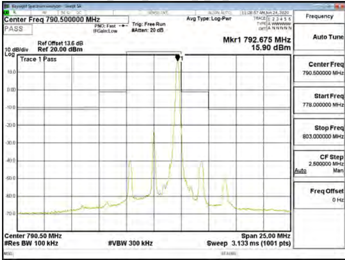
Band14_5MHz_256QAM_1_24_CH23330
