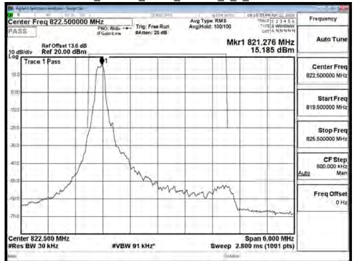
Band26_Part90s_3MHz_16QAM_1_0_CH26775
