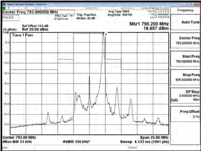
Band14_5MHz_16QAM_1_24_CH23355
