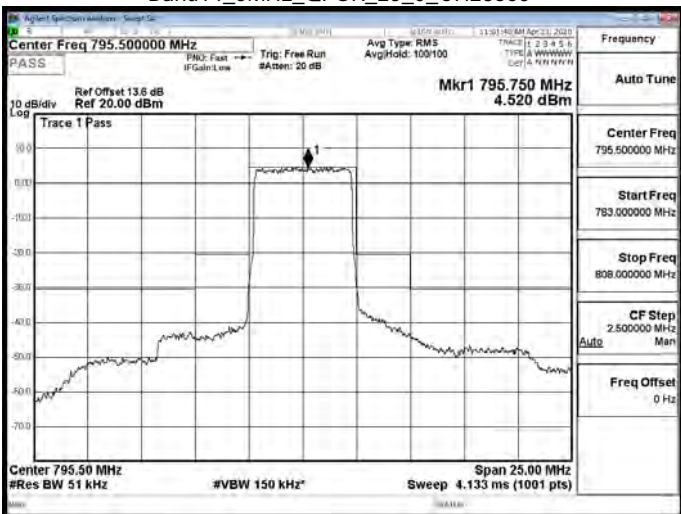
Band14_5MHz_QPSK_25_0_CH23355
