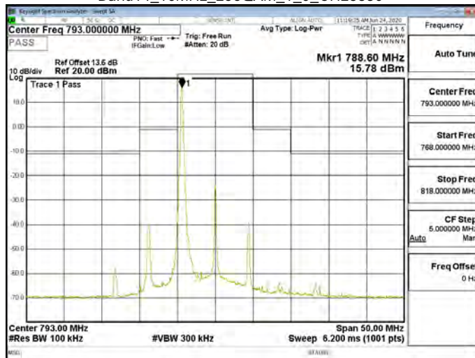
Band14_10MHz_256QAM_1_49_CH23330
