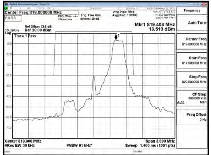
Band26_Part90s_1.4MHz_64QAM_1_5_CH26783
