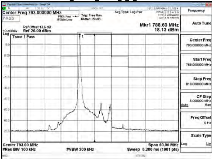
Band14_10MHz_QPSK_1_49_CH23330
