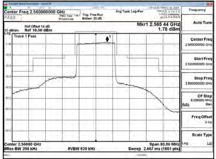
Band7_20MHz_16QAM_100_0_CH21350
