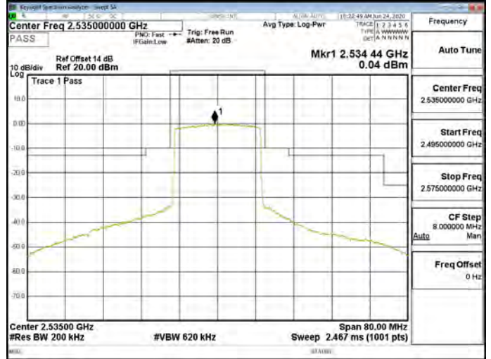
Band7_20MHz_256QAM_100_0_CH21350
