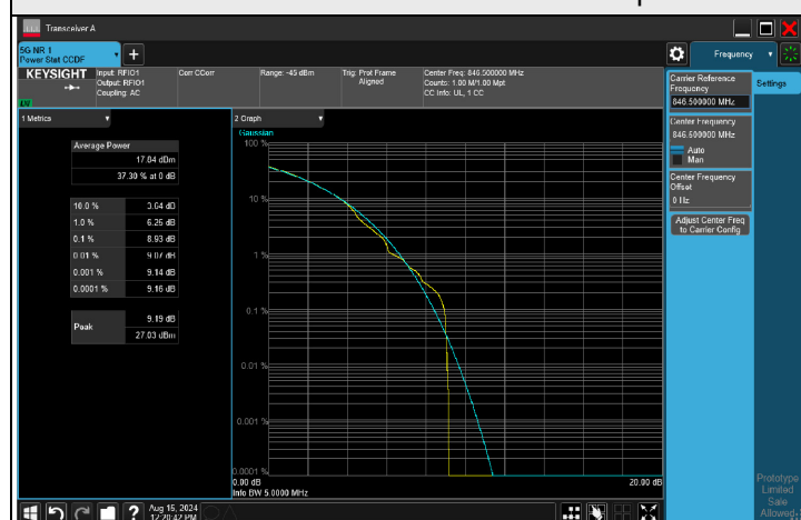
256QAM CH 169300 (846.5 MHz)
