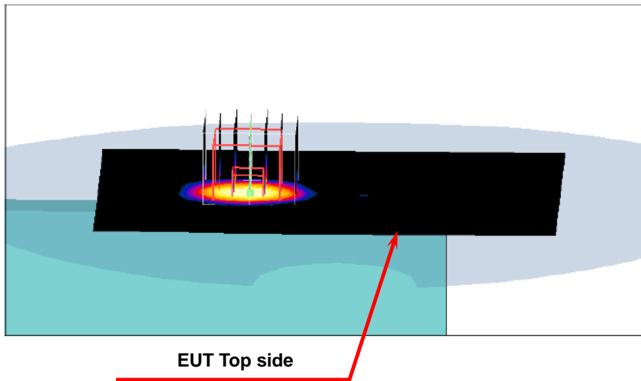
Figure 1. Body SAR Test Setup (Top Close Body)
