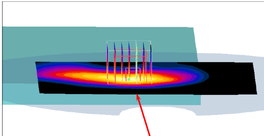
Figure 2. Body SAR Test Setup (Back Close Body)
