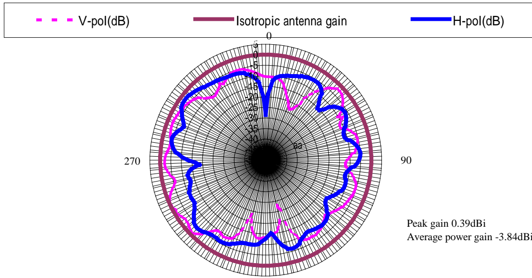
KUC Ceramic antenna radiation pattern @2.45GHz
