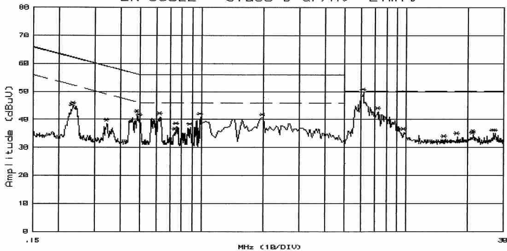
C&C Lab. Co. Shielded Room4 EN 55022 - Class B QP/AU Limit
