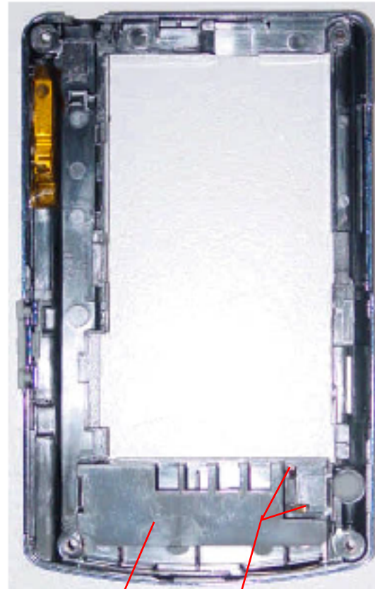
GSM Antenna Connections Antenna in Housing
