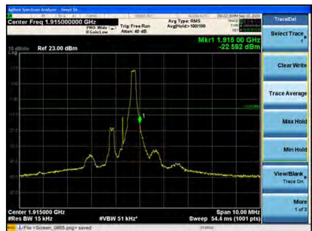
LTE Band 25 1.4MHz 16QAM 1RB CH-High
