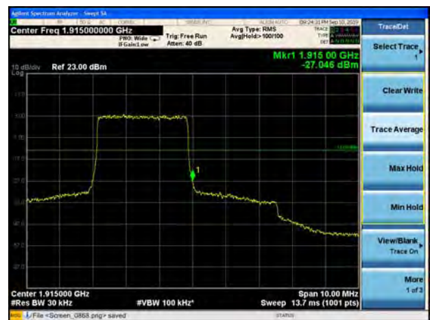
LTE Band 25 3MHz QPSK 100%RB CH-High
