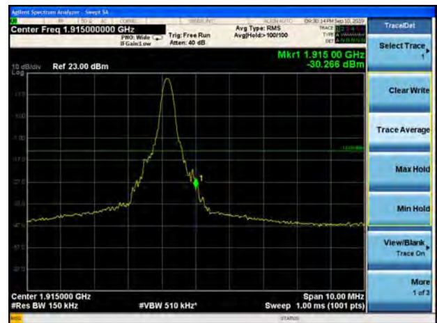
LTE Band 25 15MHz QPSK 100%RB CH-High
