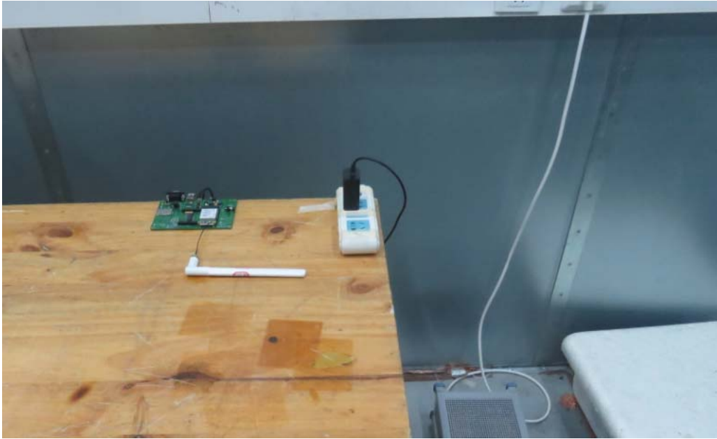
Picture 2 Conducted Emission Test Setup
