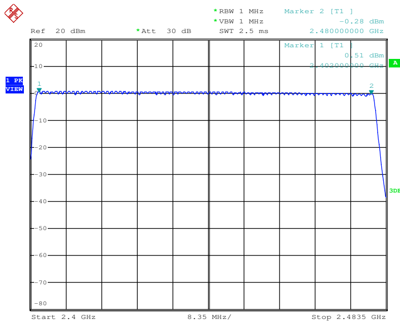
Number of Hopping Channel Plot on BR (GFSK) / Channel 0~78 / 2402 MHz ~ 2480 MHz
