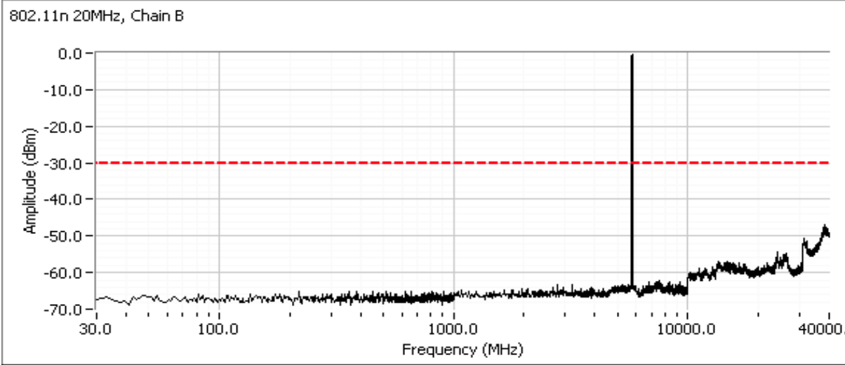
Plots for high channel, 802.11n 20MHz mode Chains A and B, power setting(s) = 28.5/27
