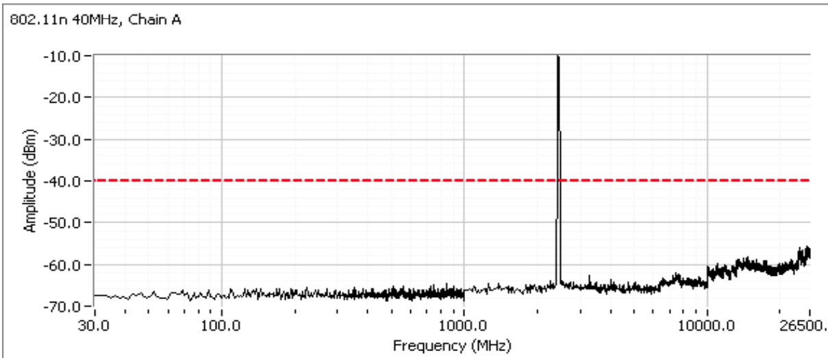
Plots for high channel, 802.11n 40MHz mode Chains A and B, power setting(s) = 22/21
