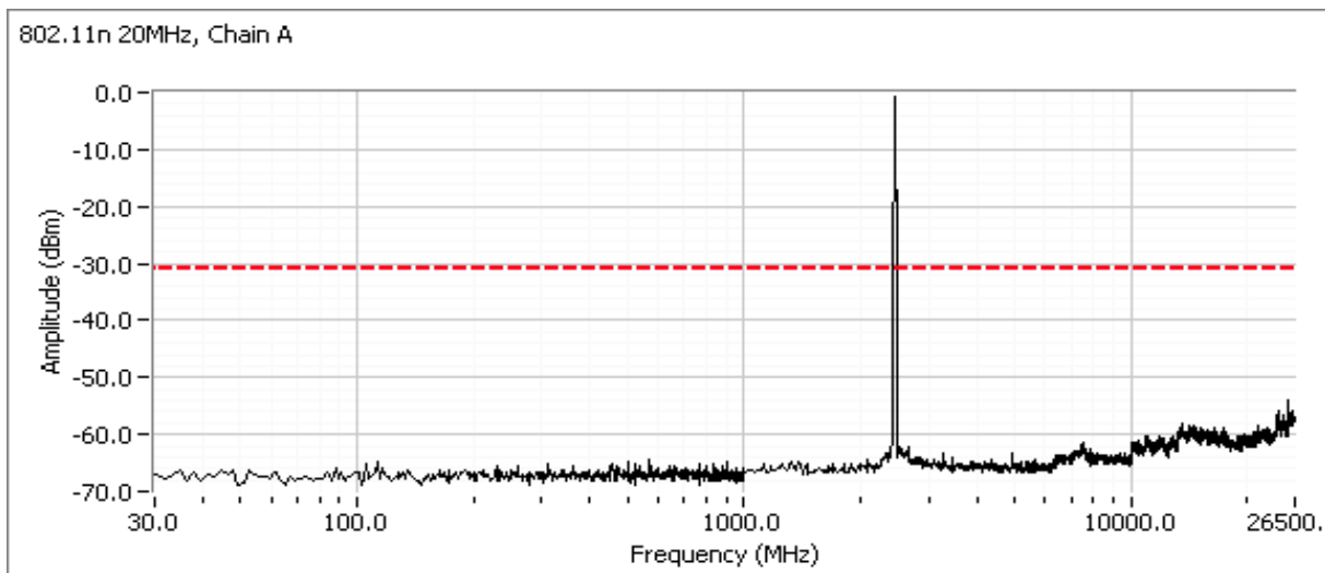
Plots for high channel, 802.11n 20MHz mode Chains A and B, power setting(s) = 26.5/25.0
