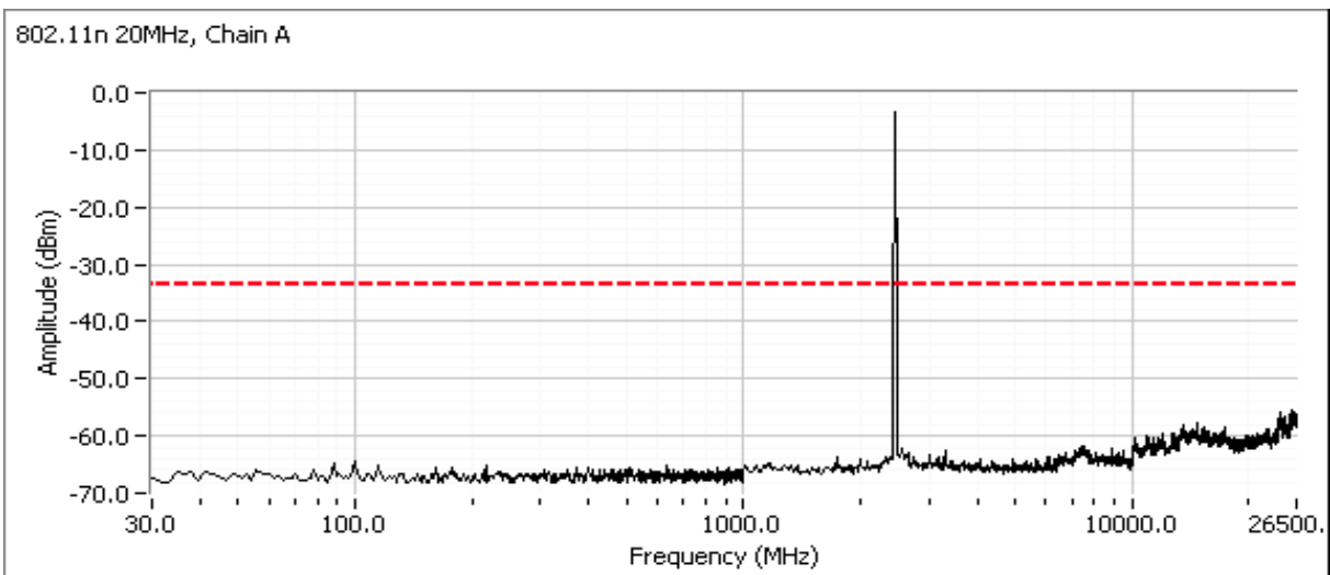
Plots for high channel, 802.11n 20MHz mode Chains A and B, power setting(s) = 25.0/24.0
