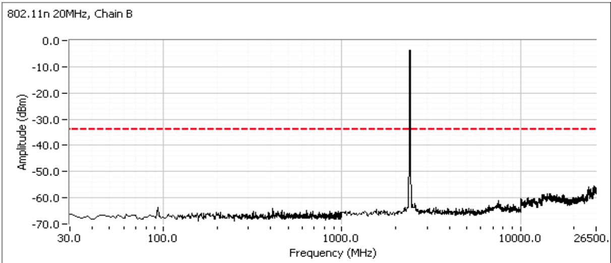
Plots for center channel, 802.11n 20MHz mode Chains A and B, power setting(s) = 29.5/28
