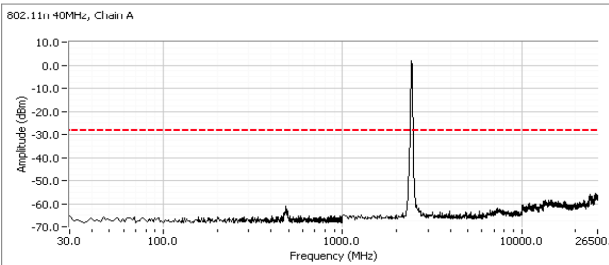
Plots for center channel, 802.11n 40MHz mode Chains A and B, power setting(s) = 29.5/28
