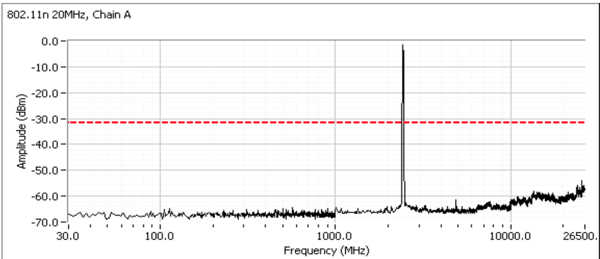
Plots for center channel, 802.11n 20MHz mode Chains A and B, power setting(s) = 31/29.5
