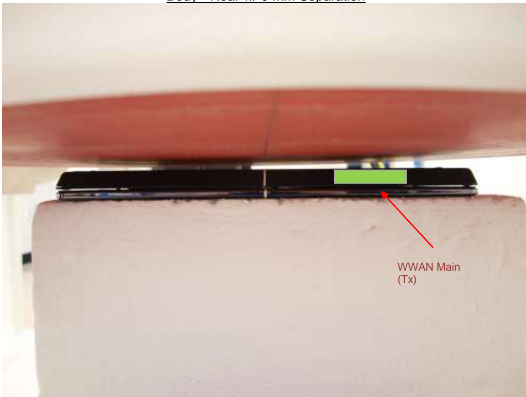
Body - Rear w/ 10 mm Separation
