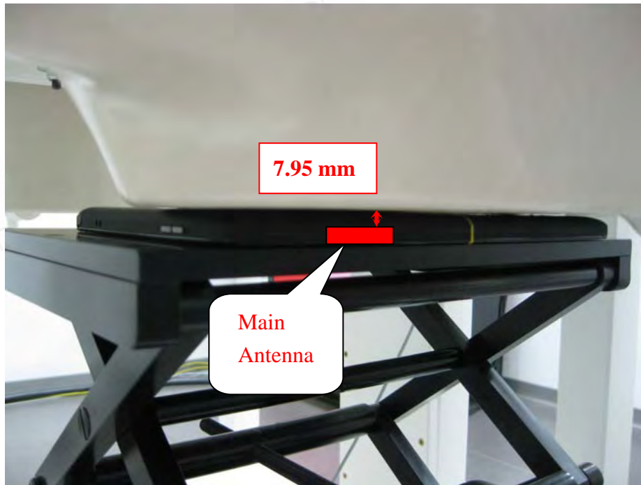
Fig.3.1 Lap-held mode (Main antenna)
