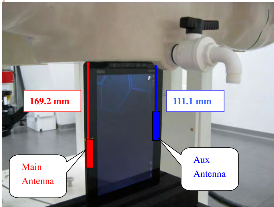
Fig.4 Primary Landscape mode
