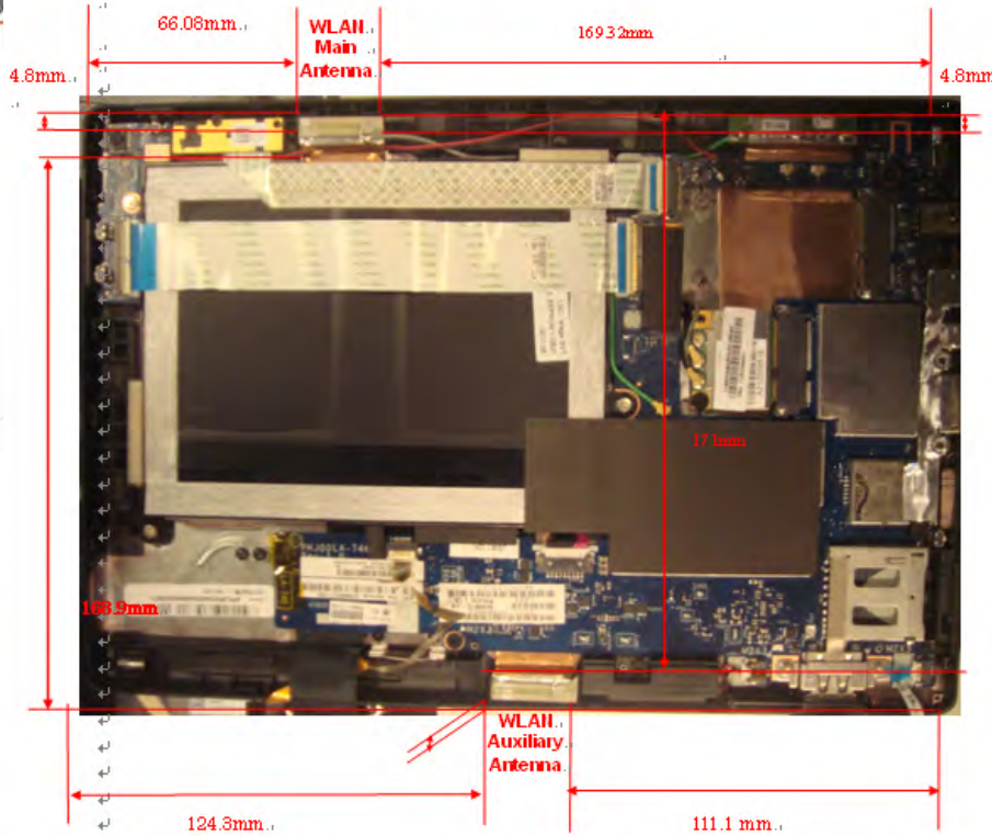
Fig.8 Antenna position & distance (Front view)
