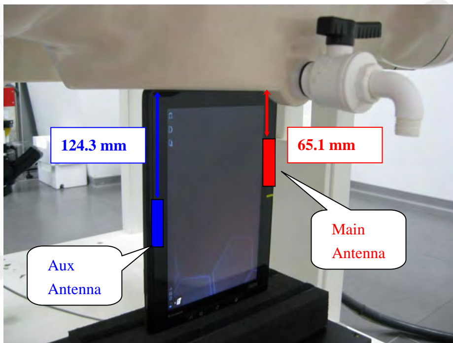
Fig.5 Secondary Landscape mode
