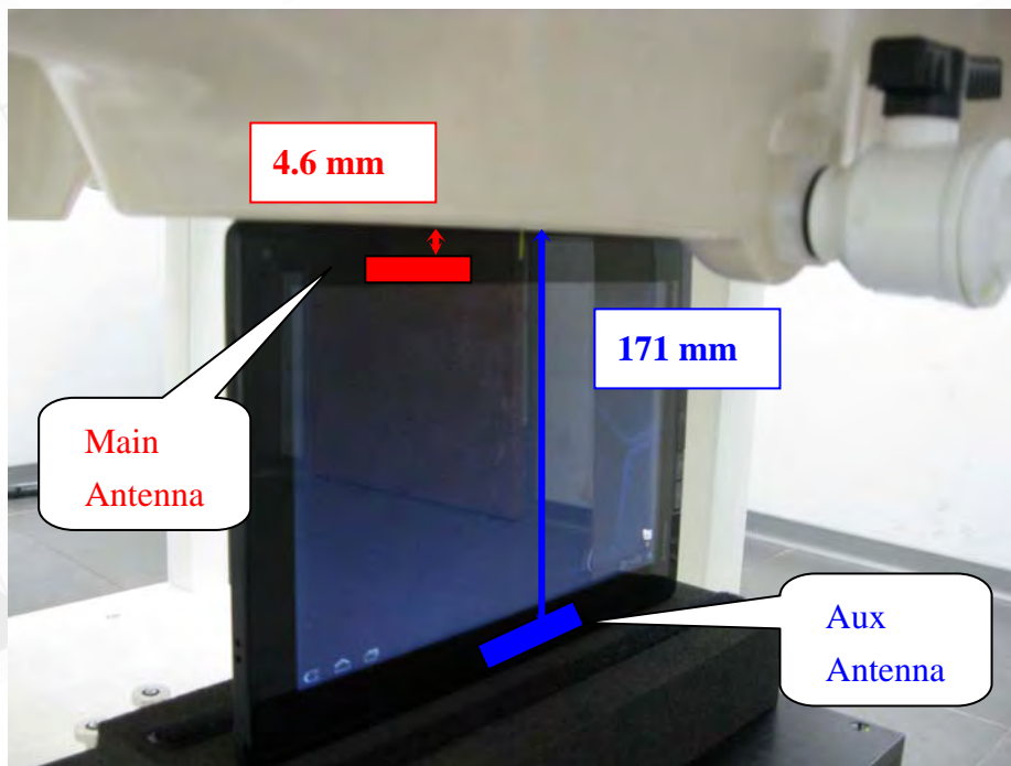
Fig.7 Secondary Portrait mode
