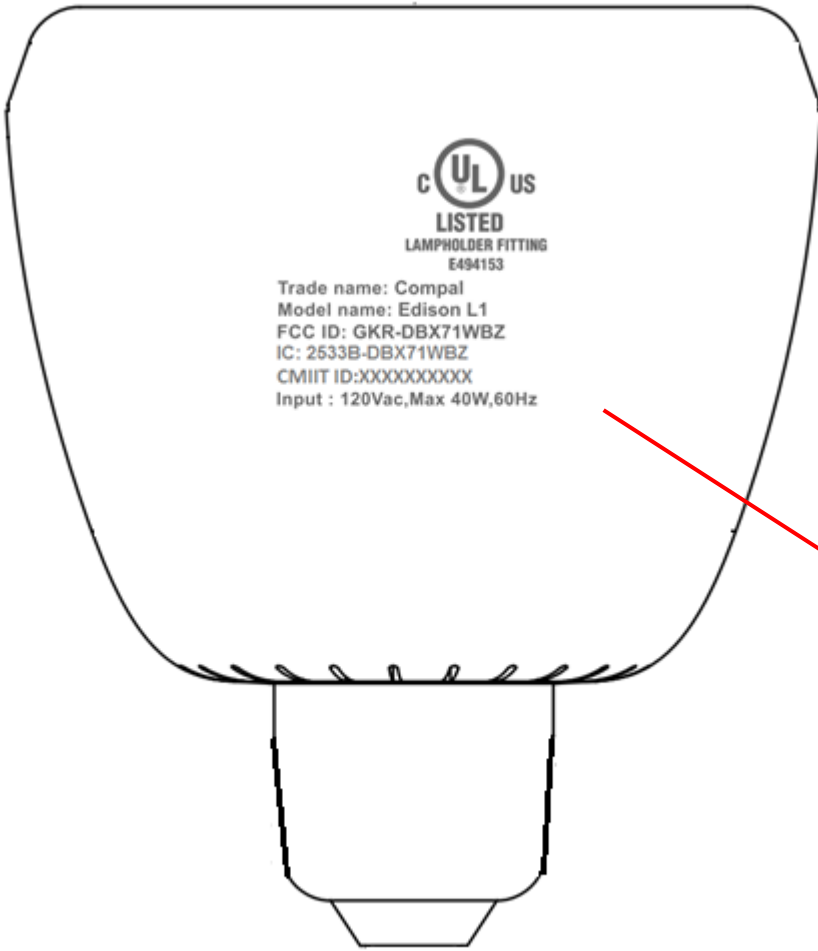
Back View
