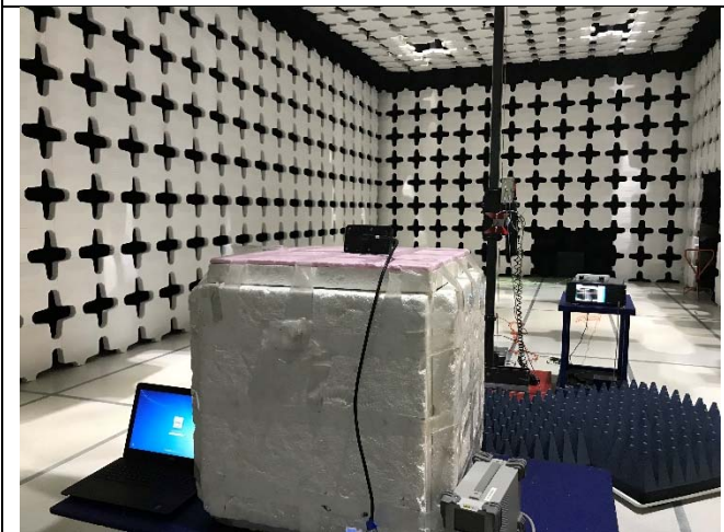
Radiated Emissions (Above 1 GHz) Front View
