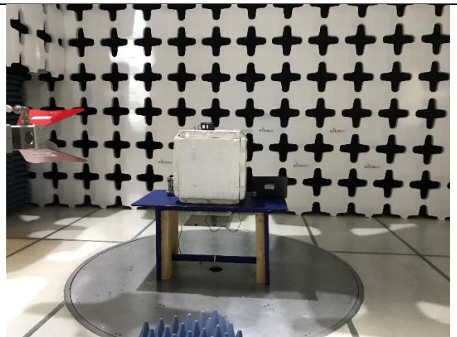
Radiated Emission (Above 1 GHz) Rear View
