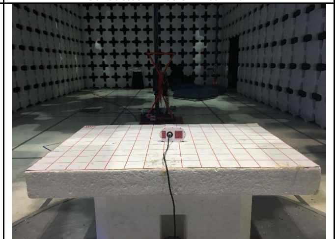
Radiated Emission Below 1G - Rear View
