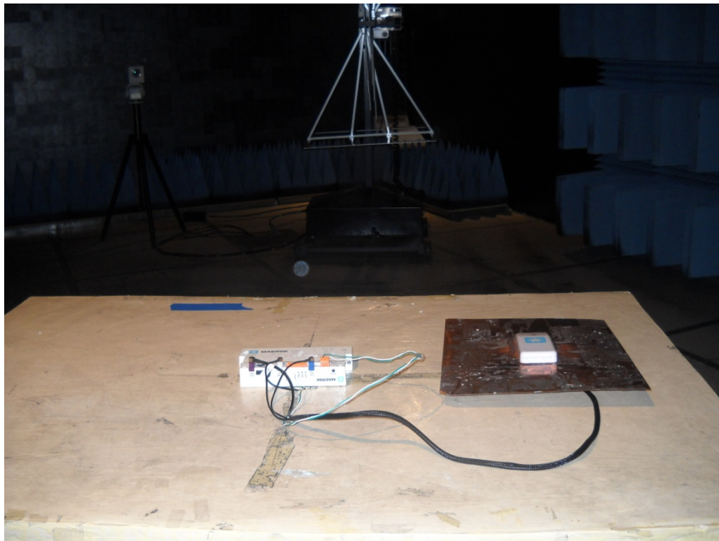
Fig. 6 Field Strength Measurements <1GHz
