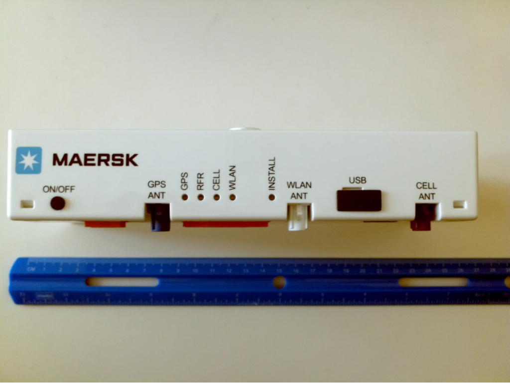
Fig.4 Front View
