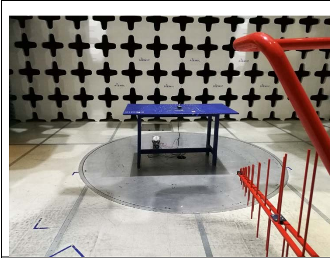
EUT Radiated Emissions (<1GHz) - Front View
