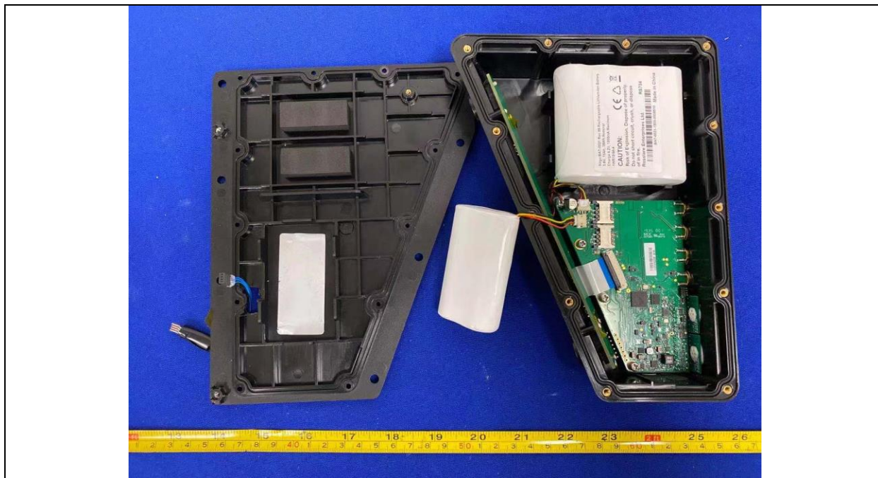
EUT Open Case View
