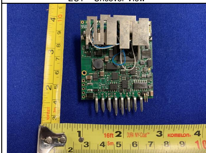
PCB Rear View
