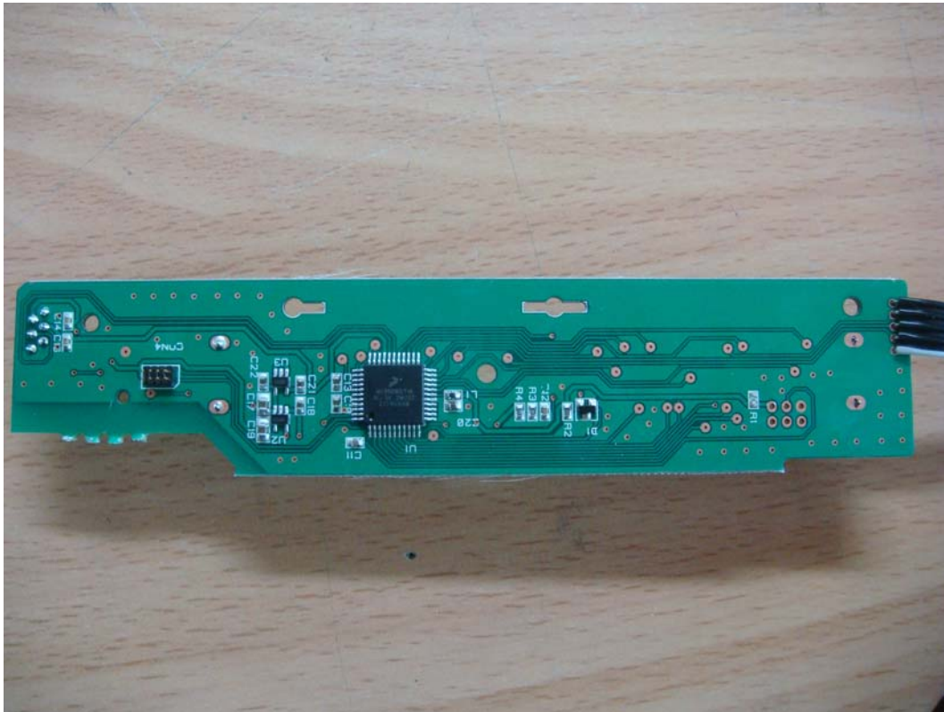
<Photograph 2: Main board - Front view>
