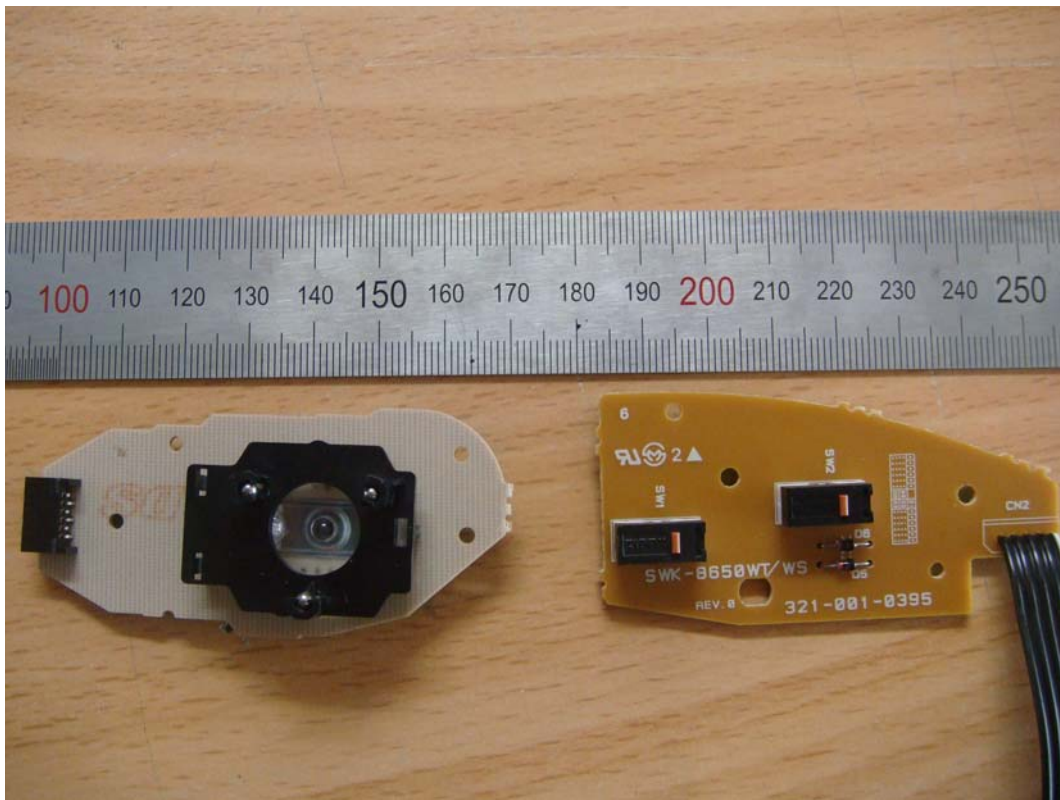
<Photograph 4: Mouse track ball & buttons - Front view>
