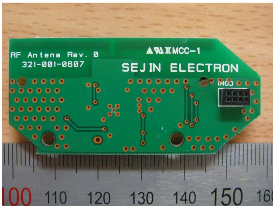
<Photograph 7: Internal RF Board - Rear view>
