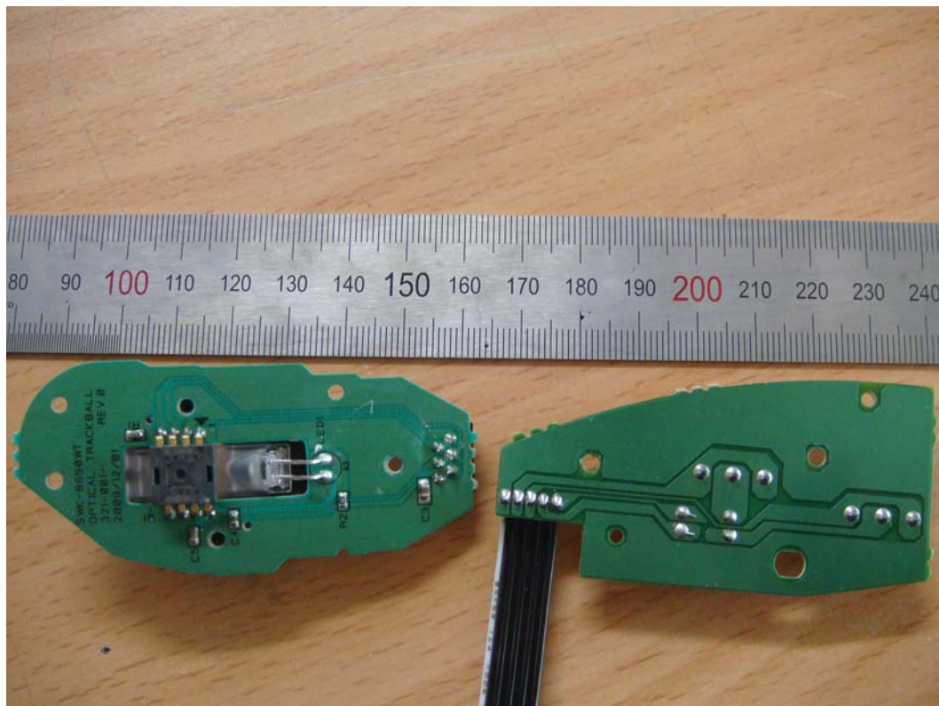
<Photograph 5: Mouse track ball & buttons - Rear view>
