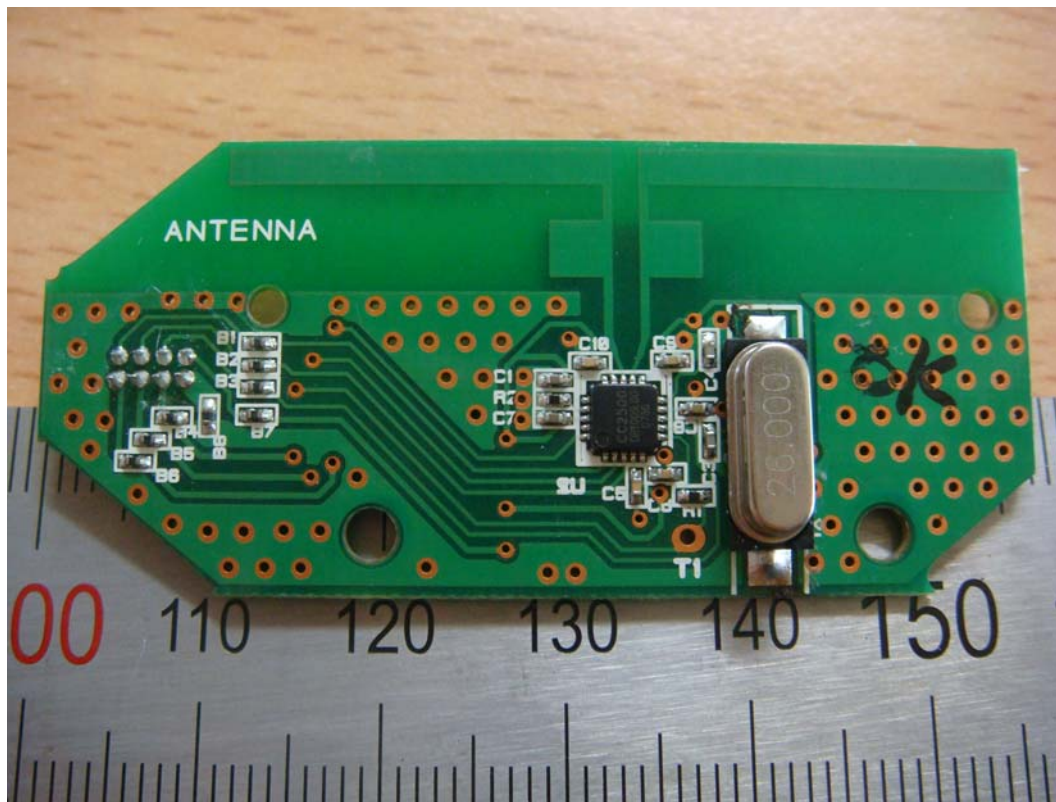
<Photograph 6: Internal RF Board - Front view>
