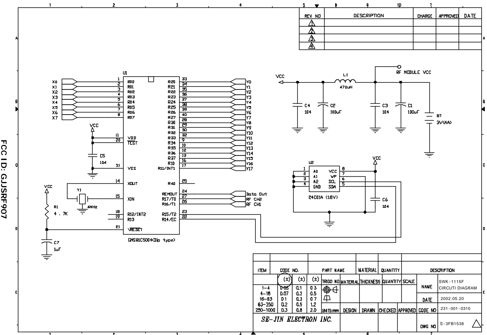
Keyboard Main board
