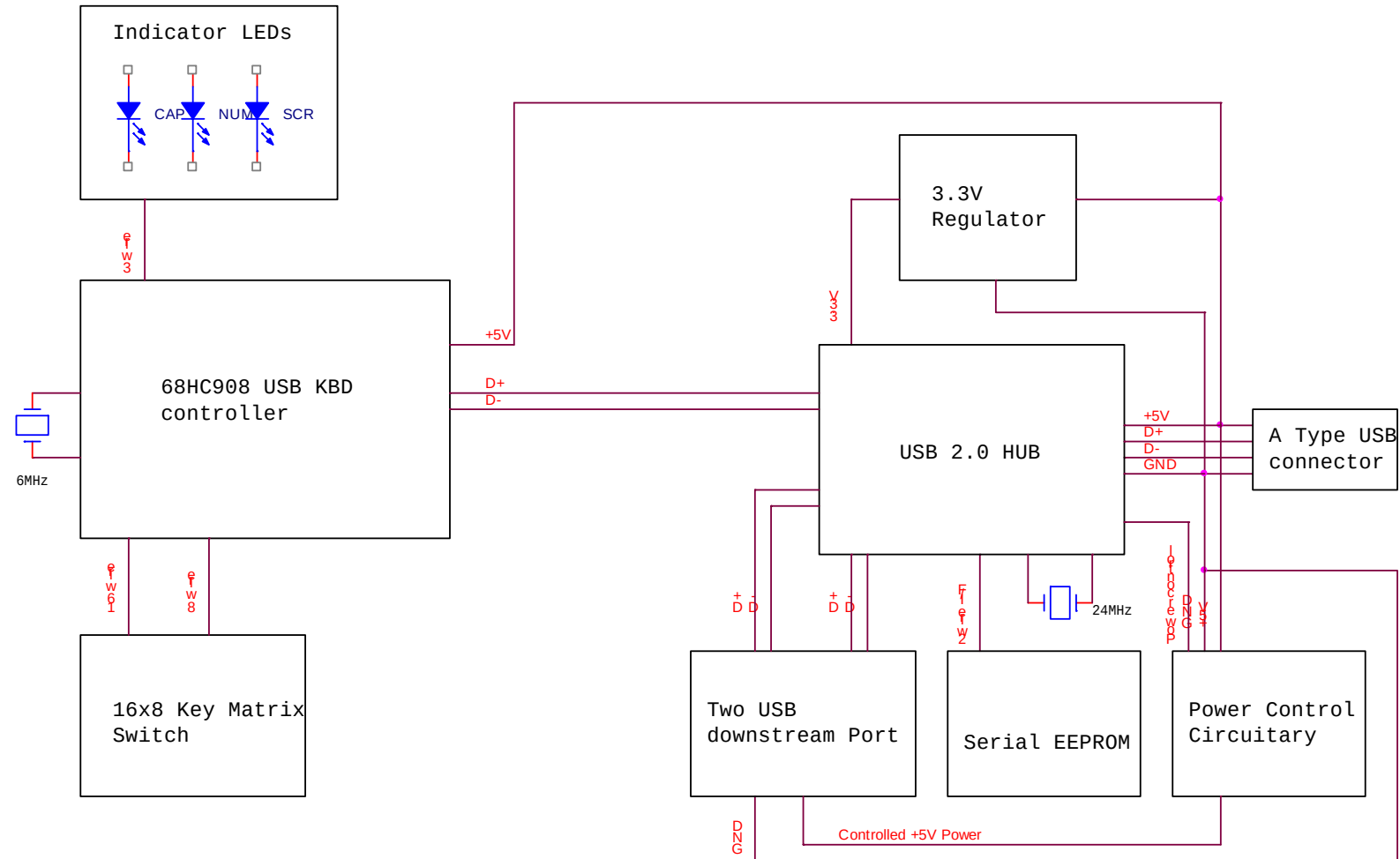
SPR-8695TUH Keyboard Block Diagram
