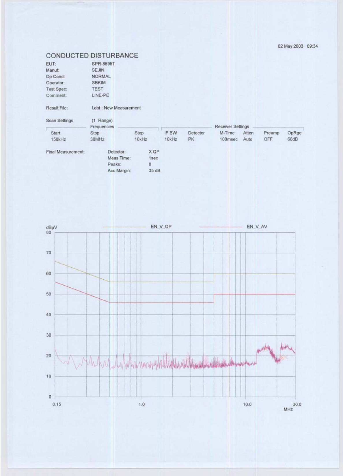
Figure 1 : Spectral Diagram, LINE - PE
