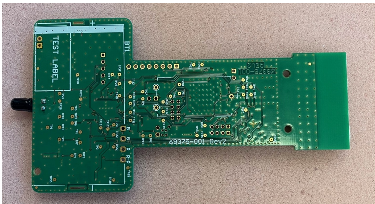
Figure 2 PCBA battery side.
