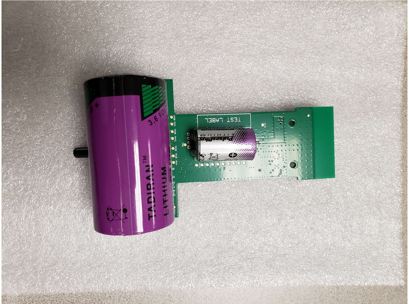
Figure 3 Batteries installed on PCBA.
