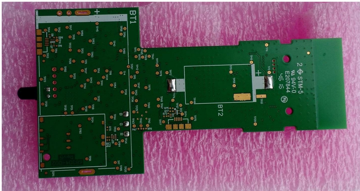
Figure 2 PCBA battery side.
