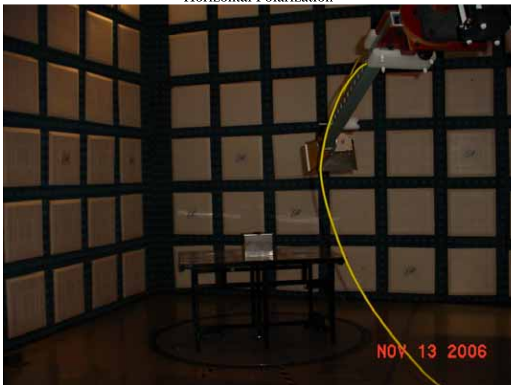
Test Setup for Radiated Emissions, 1GHz to 10GHz, with metal enclosure – Vertical Polarization
