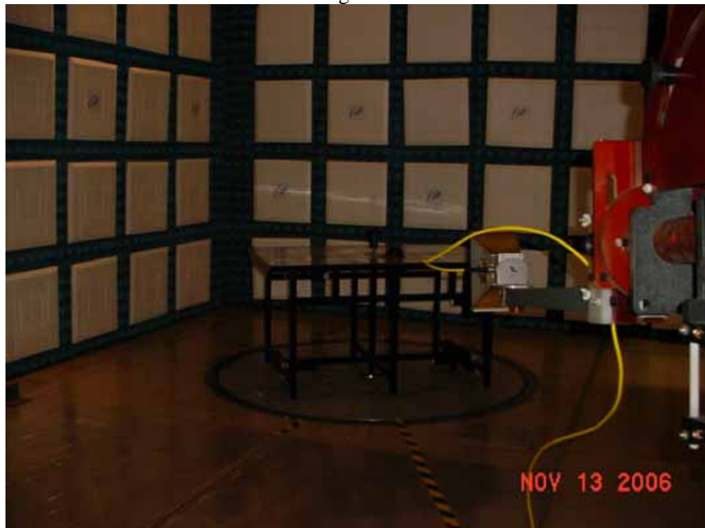
Test Setup for Radiated Emissions, 1GHz to 10GHz, with no metal enclosure – Horizontal Polarization
